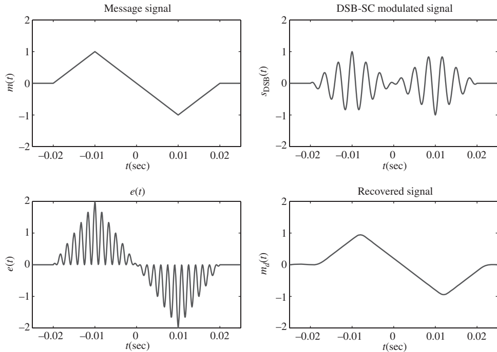
Figure 4.42 Time domain signals during DSB-SC modulation and demodulation.
