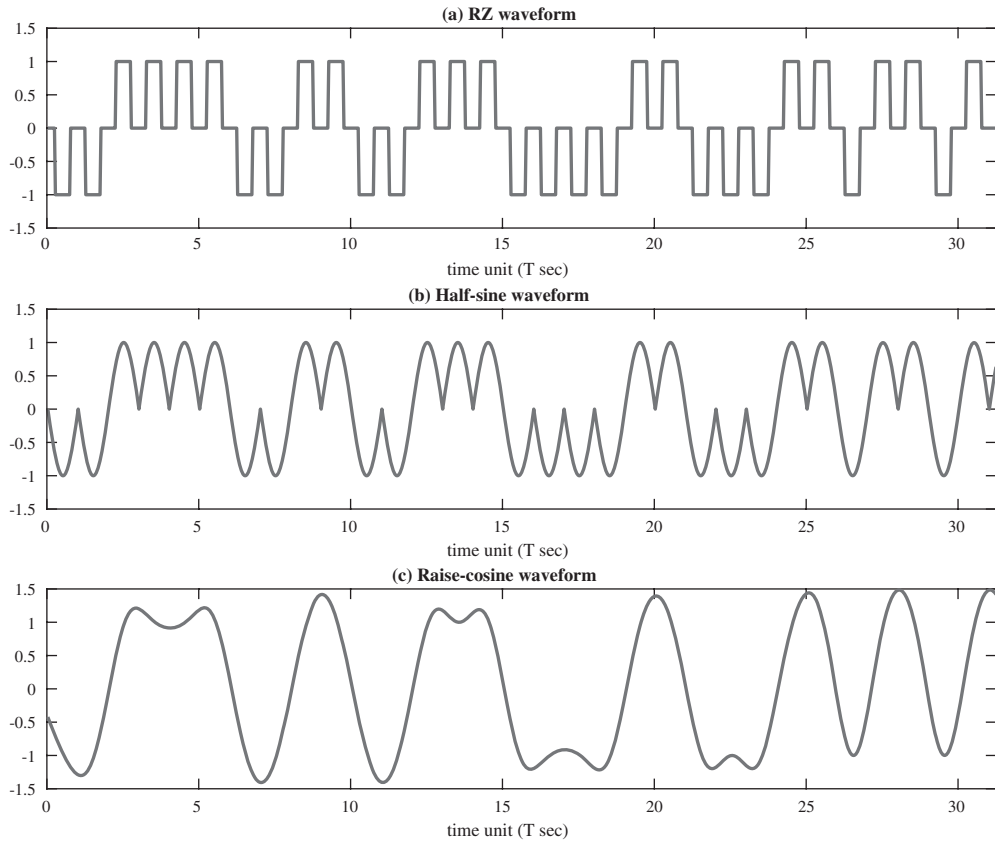
Figure 6.39 Baseband modulation signals using the following pulse shapes: (a) half-width RZ rectangular pulse; (b) half-sine pulse; (c) raised-cosine pulse with roll-off factor of 0.5.
