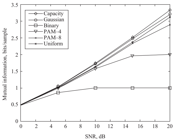
Figure 12.14 Channel capacity compared with mutual information between channel output and different input signals.
