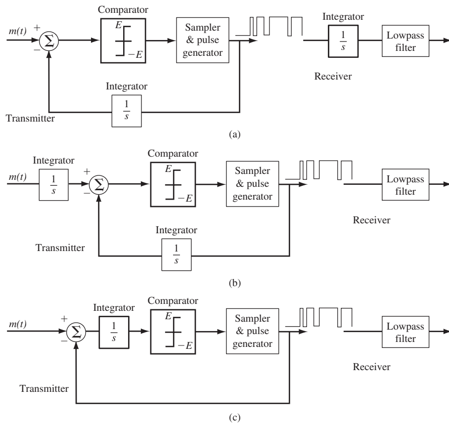
Figure 5.33 (a) Conventional delta modulator. (b) \Sigma - \Delta modulator. (c) Simpler \Sigma - \Delta modulator.
