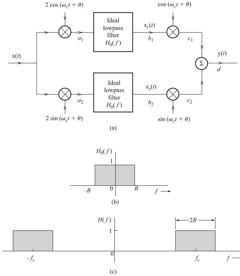
Figure 8.22 (a) Equivalent circuit of an ideal bandpass filter. (b) Ideal lowpass filter frequency response. (c) Ideal bandpass filter frequency response.
