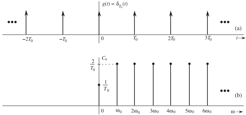
Figure 2.22 (a) Impulse train and (b) its Fourier spectrum.
