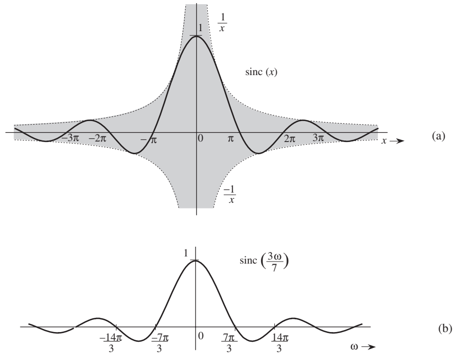
Figure 3.7 Sinc pulse.
