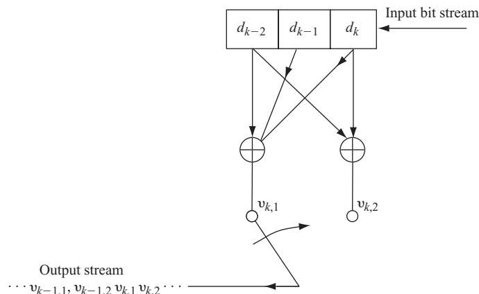
Figure 13.5 Convolutional encoder.
