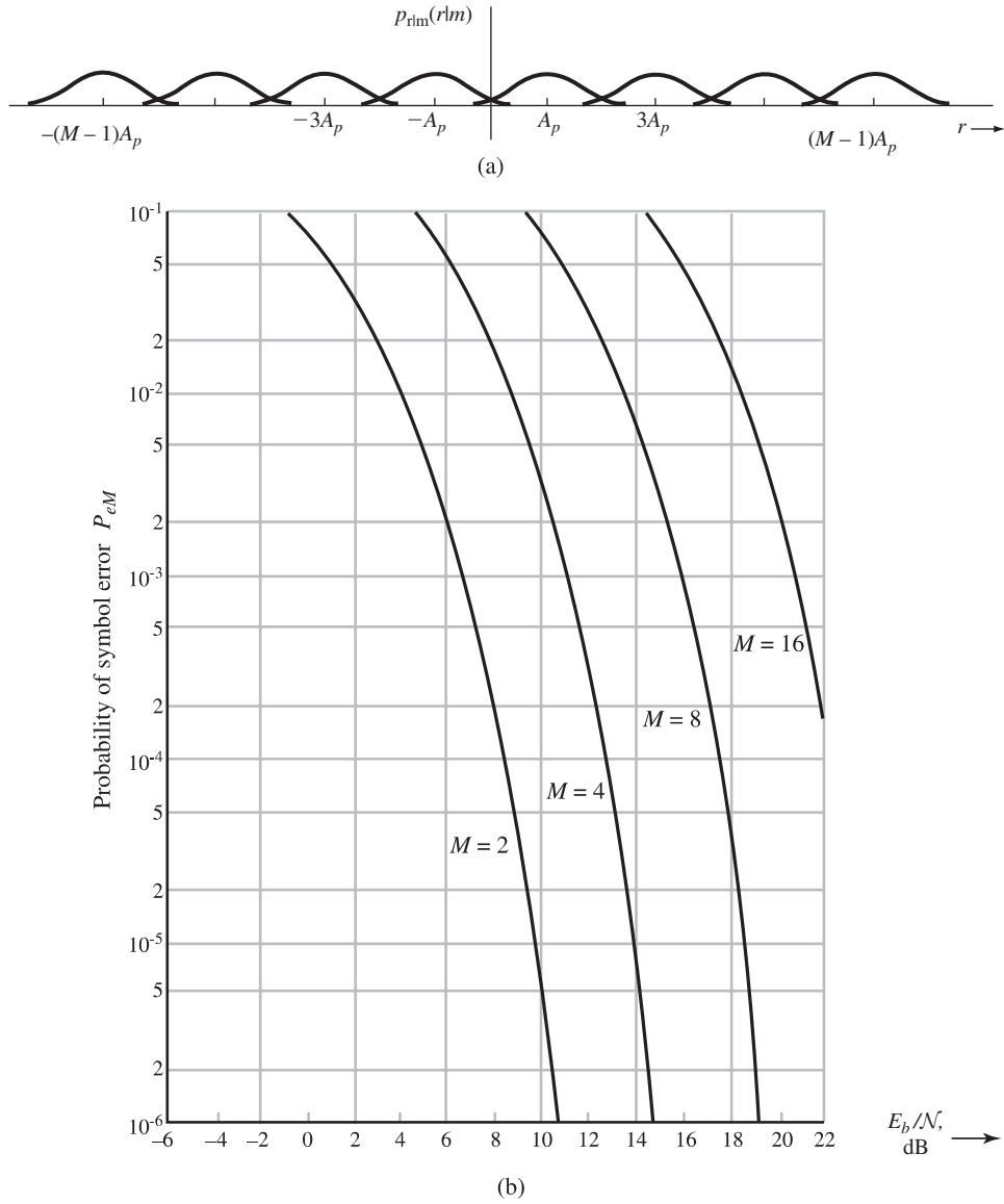
Figure 9.22 (a) Conditional PDFs in PAM. (b) Error probability in PAM.
