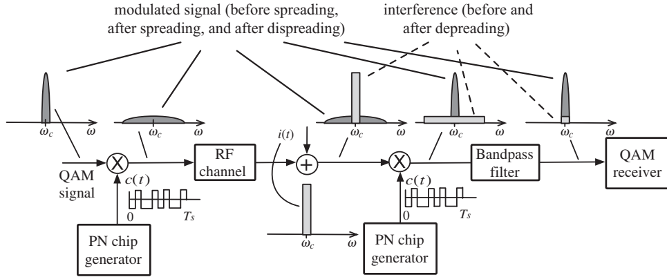
Figure 10.10 Narrowband interference mitigation by the DSSS despreader.
