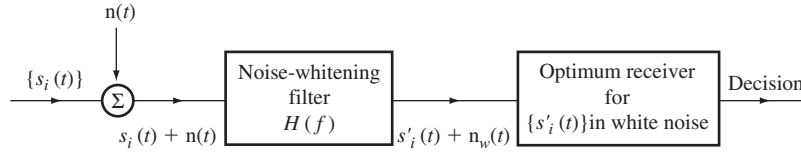
Figure 9.33 Optimum M -ary receiver for nonwhite channel noise.
