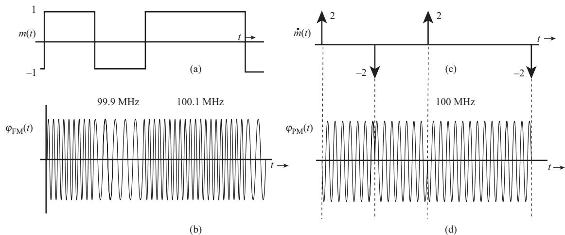
Figure 4.26 FM and PM waveforms.
