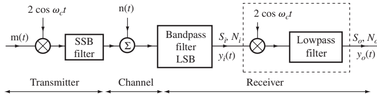
Figure 8.31 SSB-SC system.
