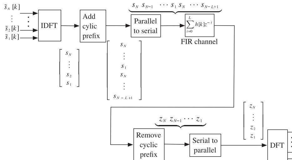
Figure 11.13 DMT transmission of N different symbol streams over a single FIR channel.
