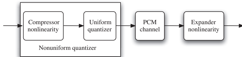
Figure 5.18 Utilization of compressor and expander for nonuniform quantization.
