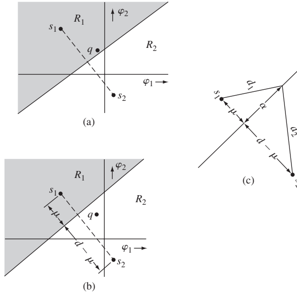
Figure 9.19 Determining optimum decision regions in a binary case.
