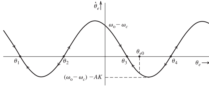
Figure 4.38 Trajectory of a first-order PLL.
