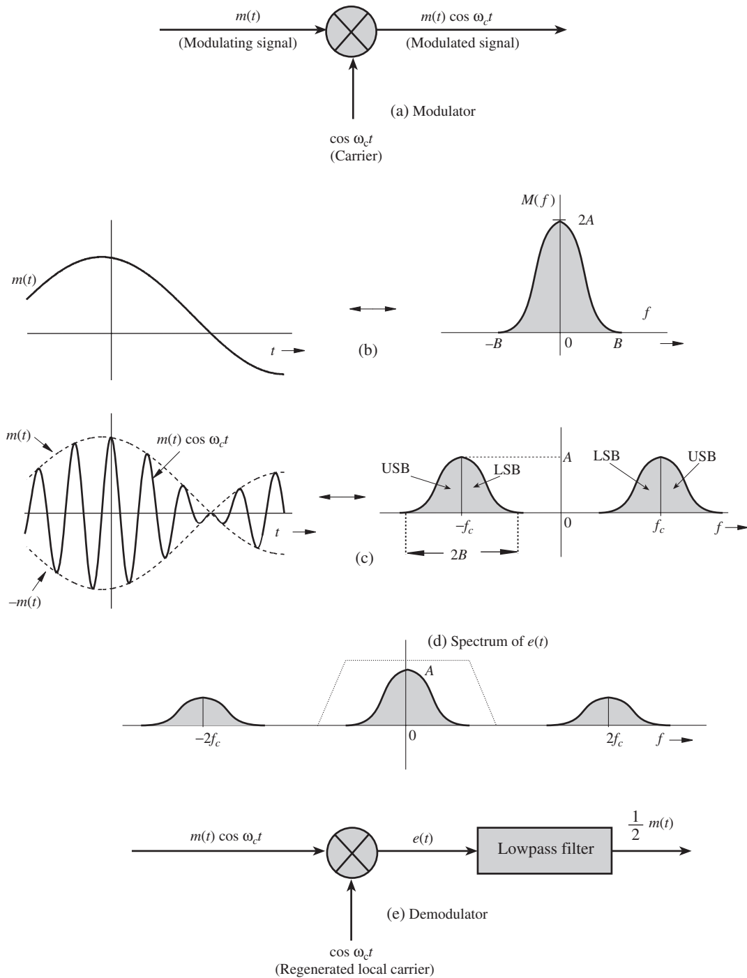
Figure 4.1 Double-sideband, suppressed-carrier (DSB-SC) modulation and demodulation.
