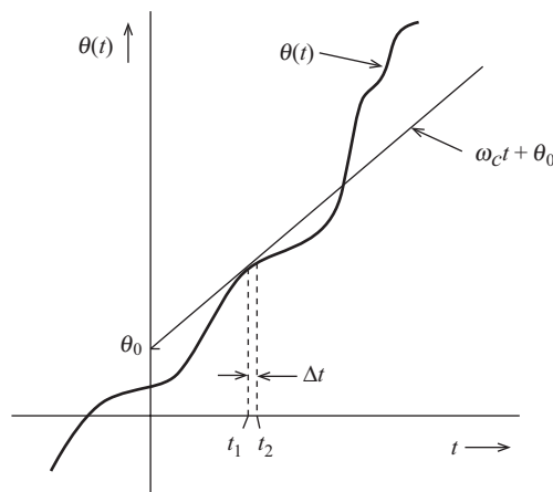
Figure 4.24 Concept of instantaneous frequency.
