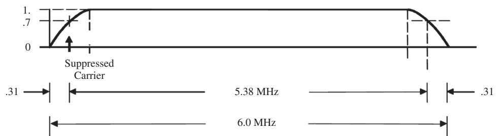
Figure 4.23 VSB spectra of ATSC transmission for HDTV over 6 MHz total bandwidth.
