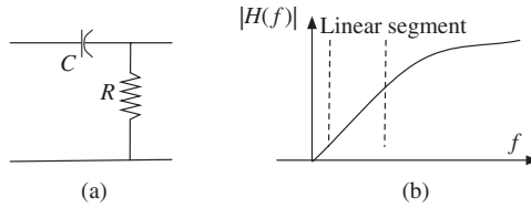
Figure 4.29 (a) RC highpass filter. (b) Segment of positive slope in amplitude response.
