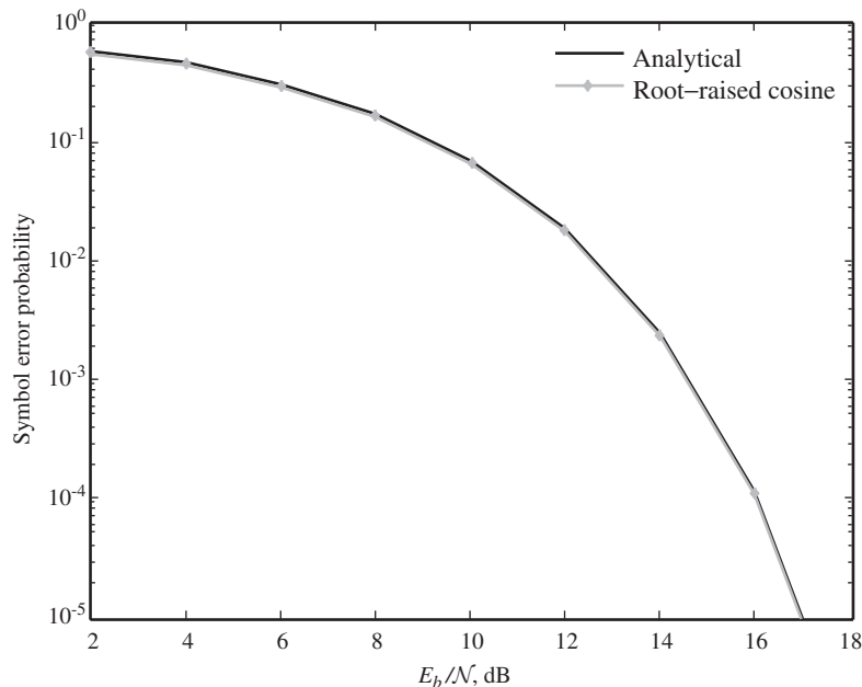
Figure 9.48 Symbol error probability of 16-QAM using root-raised cosine pulse in comparison with the analytical result.
