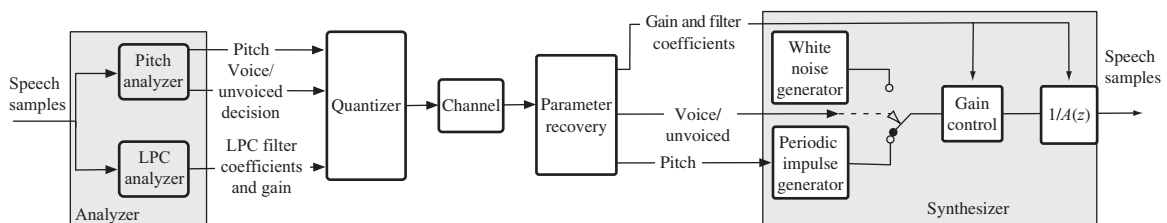
Figure 5.35 Analysis and synthesis of voice signals in an LPC encoder and decoder.
