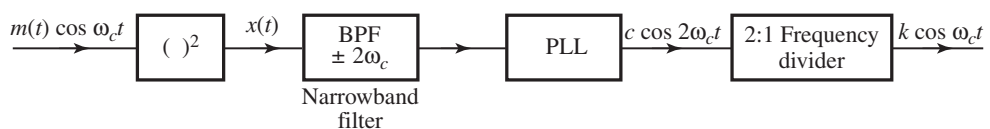
Figure 4.39 Generation of coherent demodulation carrier using signal squaring.
