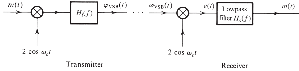
Figure 4.19 VSB modulator and demodulator.
