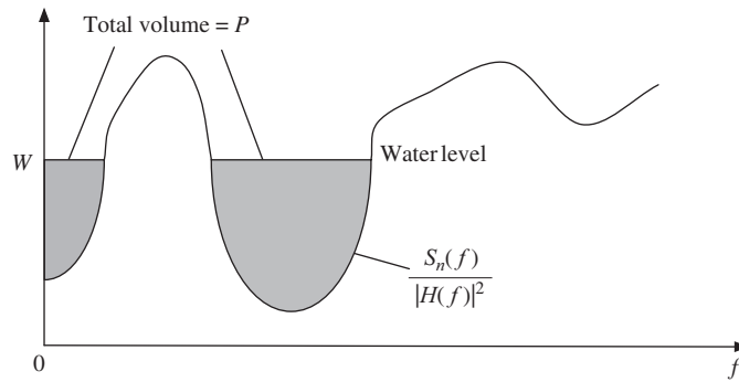
Figure 12.9 Illustration of water-pouring power allocation for maximizing frequency-selective channel capacity.
