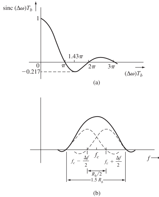
Figure 9.11 (a) The minimum of the sinc function and (b) the MSK spectrum.
