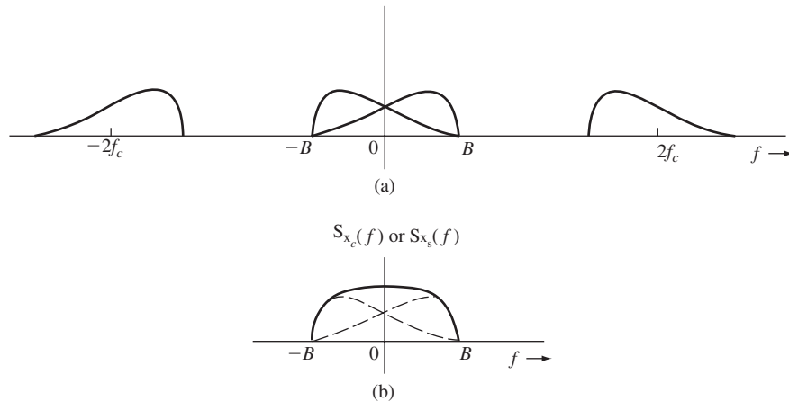
Figure 8.23 Derivation of PSDs of quadrature components of a bandpass random process.
