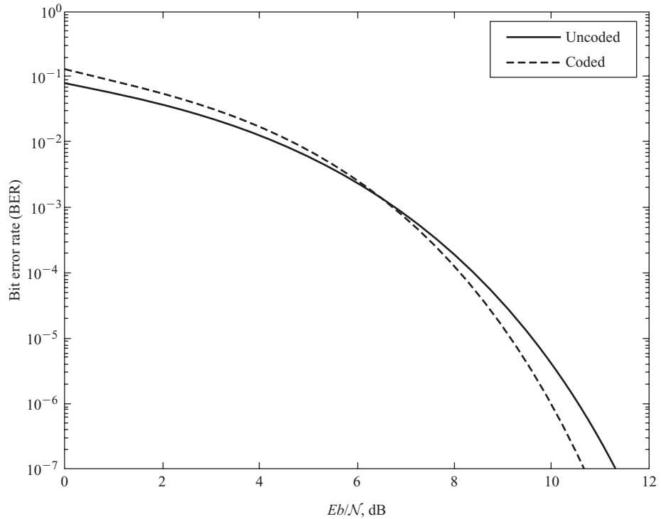
Figure 13.24 Comparison of BERs of uncoded polar signaling transmission and polar signaling transmission of Hamming (7, 4) encoded (dashed) and uncoded (solid) message bits.
