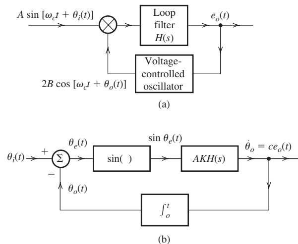
Figure 4.36 Phase-locked loop and its equivalent circuit.
