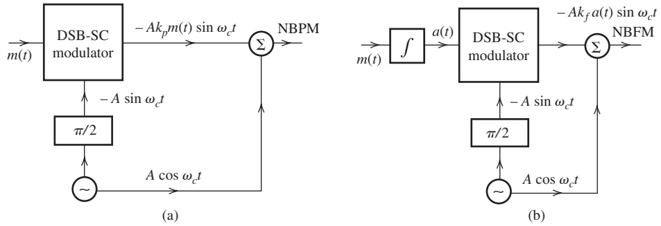
Figure 4.32 (a) Narrowband PM generator. (b) Narrowband FM signal generator.
