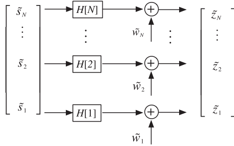
Figure 11.11 N independent AWGN channels generated by OFDM without ISI.
