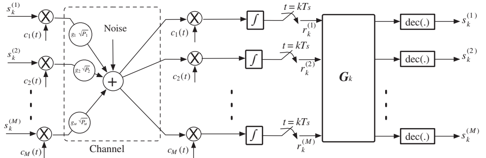
Figure 10.15 Minimum mean square error MUD receiver.
