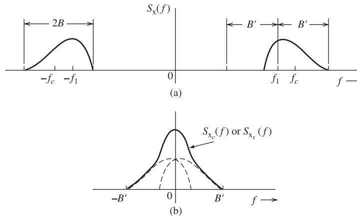
Figure 8.25 Nonunique nature of quadrature component representation of a bandpass process.
