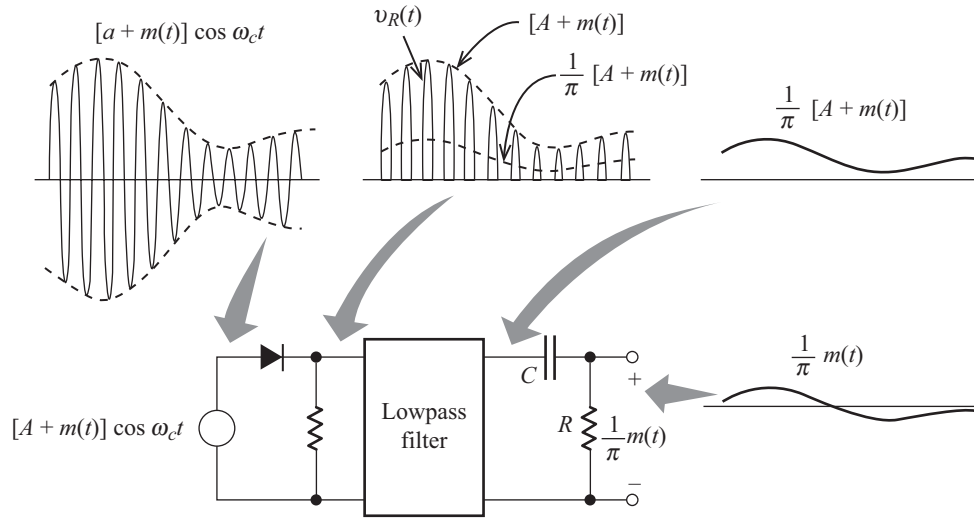
Figure 4.9 Rectifier detector for AM.
