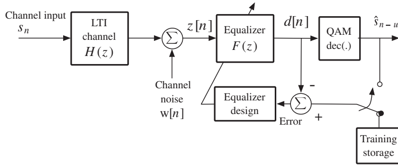
Figure 11.18 Channel equalization based on a training phase before switching to decision feedback mode.
