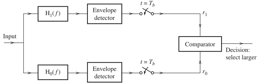
Figure 9.38 Noncoherent detection of binary FSK.
