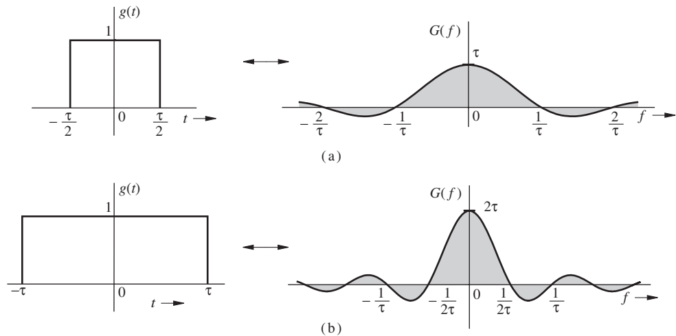
Figure 3.15 The scaling property of the Fourier transform.
