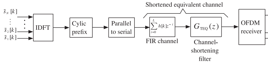
Figure 11.15 Time domain equalizer (TEQ) for channel shortening in DMT (OFDM) transmission system with N subcarriers.
