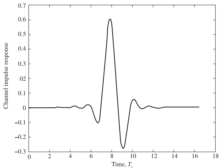
Figure 11.19 Two-ray multipath channel response for QAM transmission.
