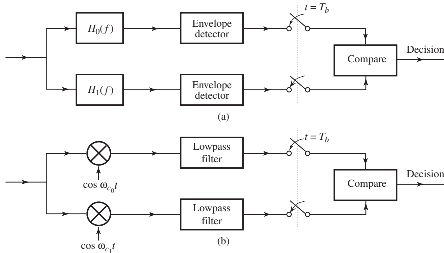
Figure 6.33 (a) Noncoherent detection of FSK. (b) Coherent detection of FSK.
