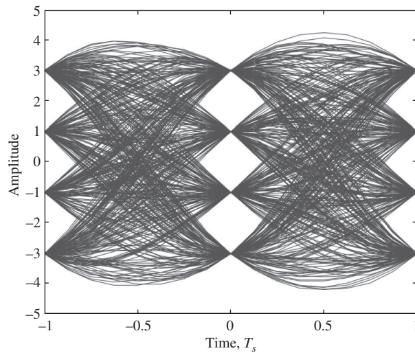
Figure 9.47 Eye diagram of the real (in-phase) component of the 16-QAM transmission at the receiver matched filter output.
