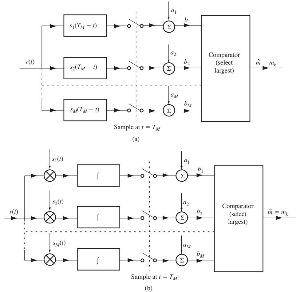
Figure 9.17 Optimum M -ary receiver: (a) matched filter detector; (b) correlation detector.
