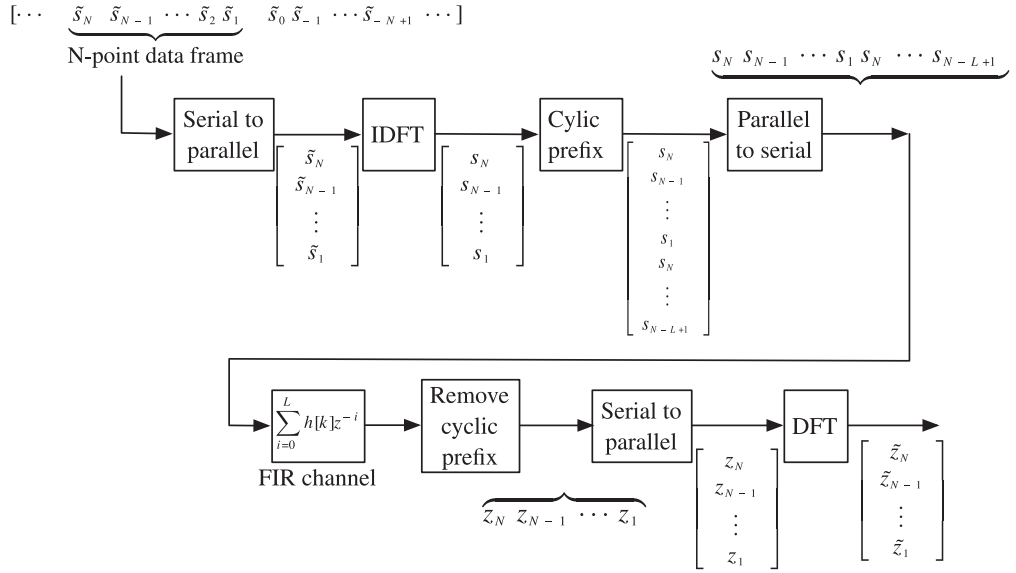
Figure 11.10 Illustration of an N-point OFDM transmission system.
