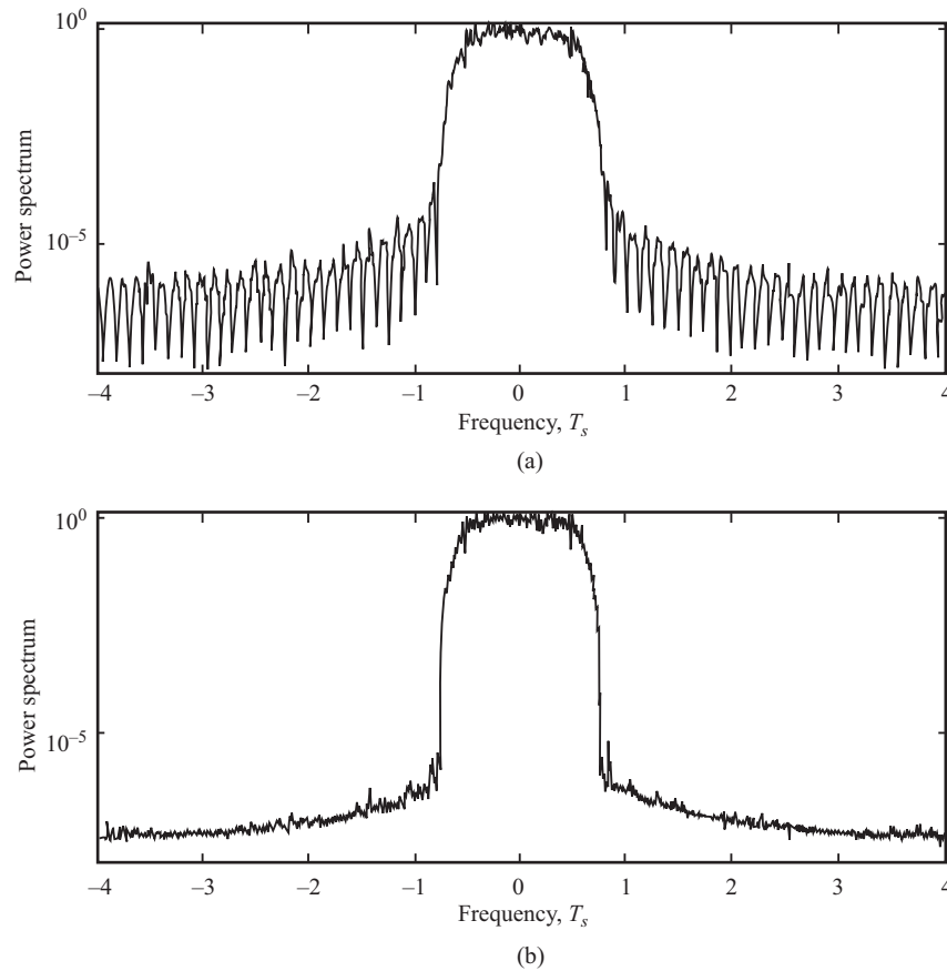
Figure 11.20 Power spectral densities of the root-raised-cosine QAM signal before and after a lowpass channel of bandwidth 0.75/T : (a) input and (b) output of lowpass filter spectra.
