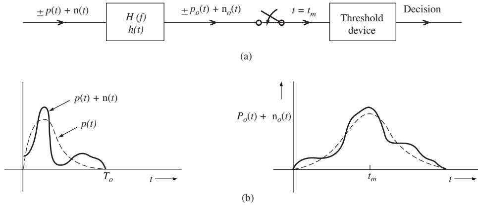
Figure 9.1 Typical binary polar signaling and linear receiver.
