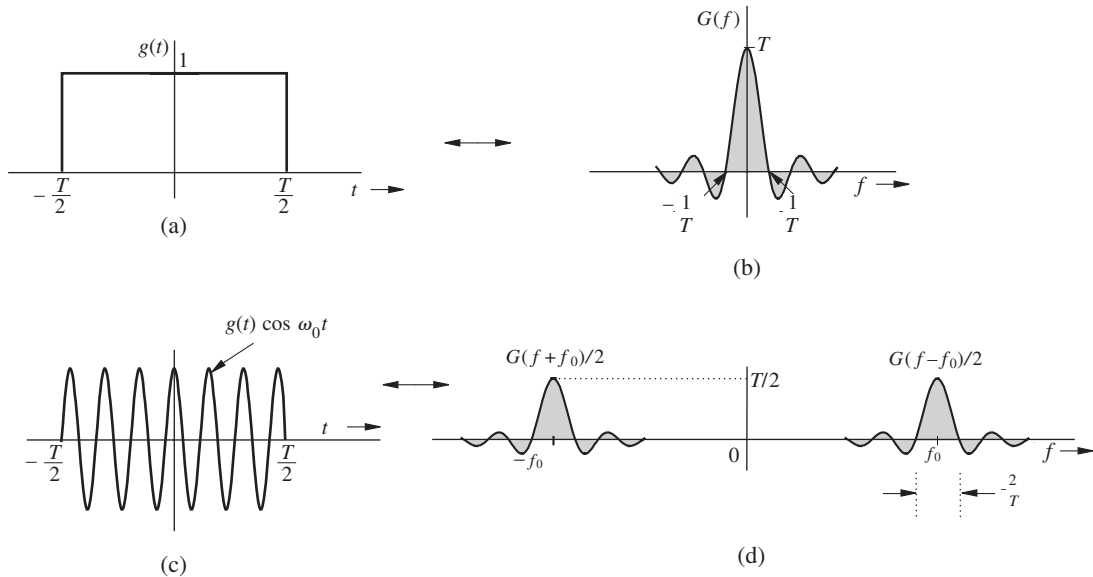
Figure 3.20 Example of spectral shifting by amplitude modulation.
