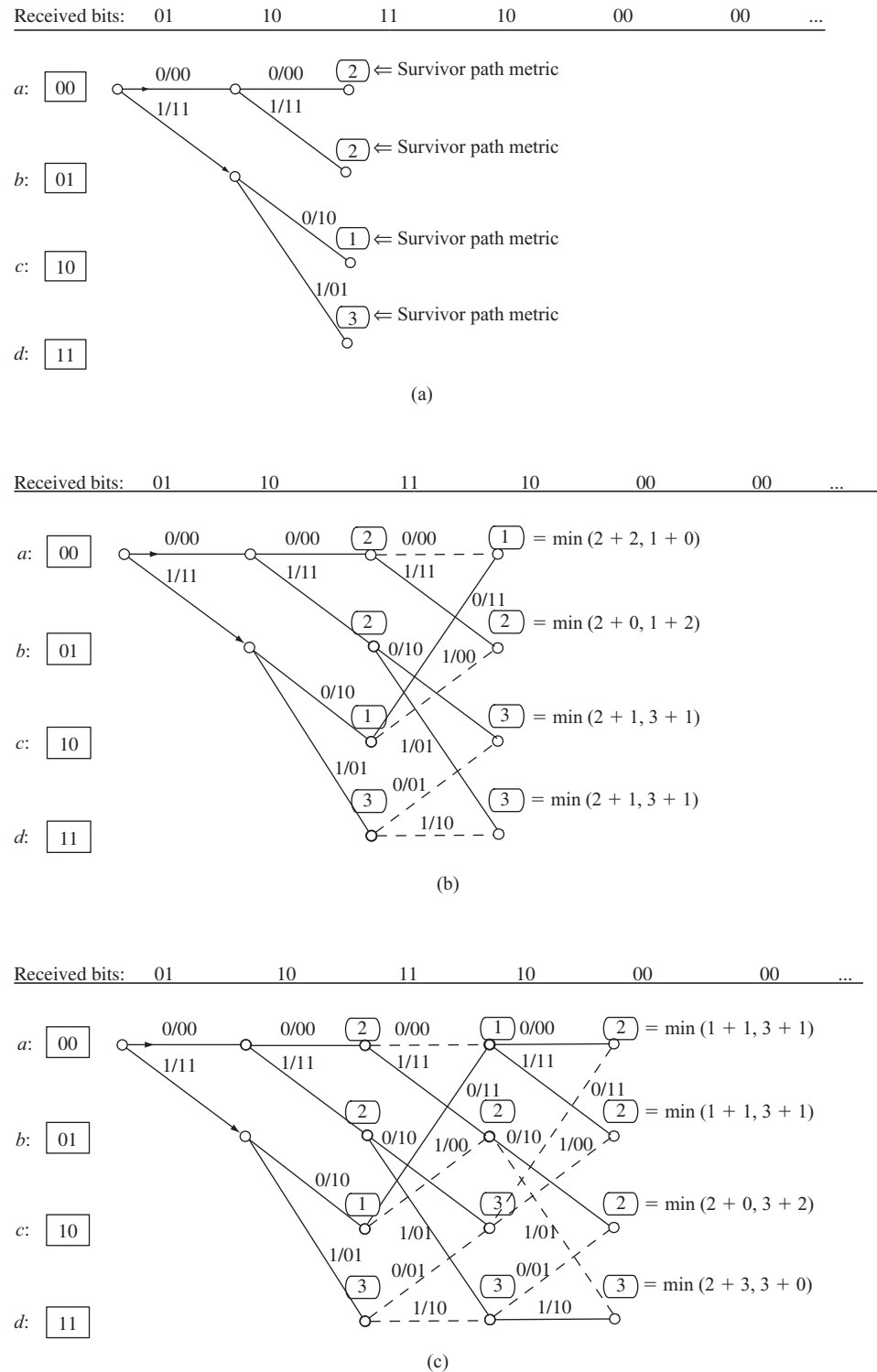
Figure 13.9 Viterbi decoding example in Fig. 13.5: (a) stages 1 and 2; (b) stage 3; (c) stage 4.
