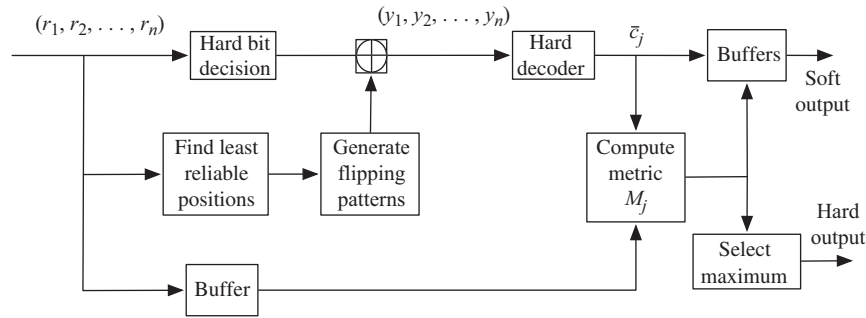
Figure 13.17 Block diagram of Chase soft-decoding algorithms.
