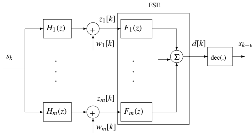
Figure 11.7 Equivalent structure of fractionally spaced equalizers (FSE).
