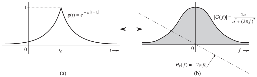
Figure 3.18 Effect of time shifting on the Fourier spectrum of a signal.
