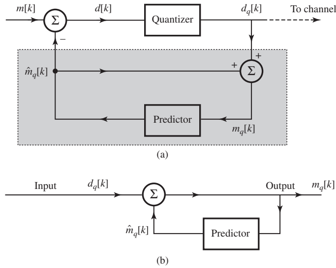
Figure 5.29 DPCM system: (a) transmitter; (b) receiver.
