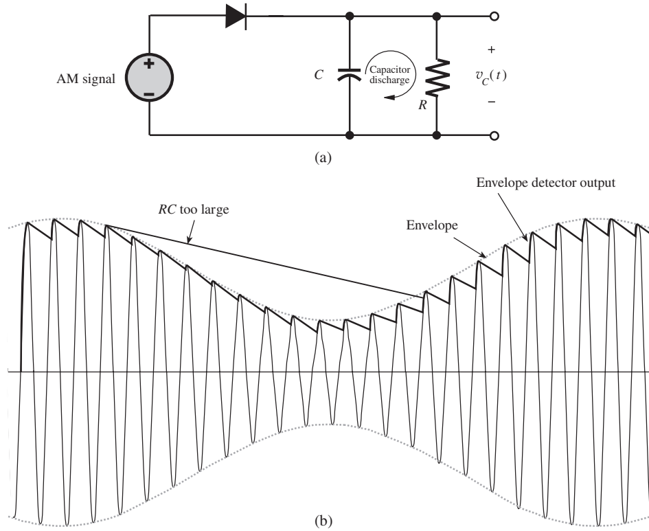
Figure 4.10 Envelope detector for AM.
