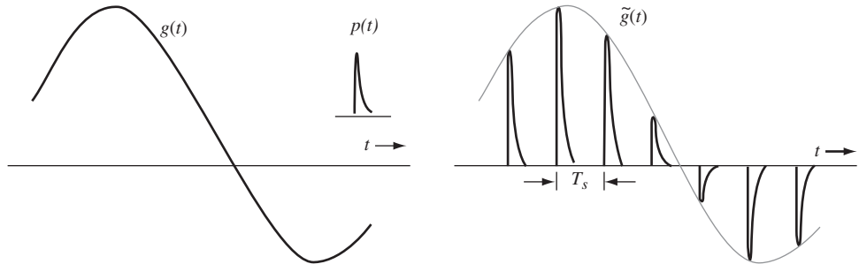
Figure 5.4 Practical reconstruction (interpolation) pulse.
