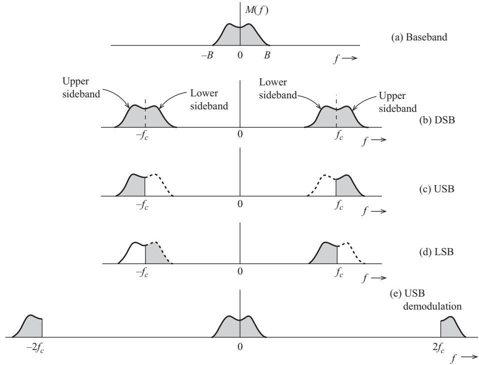
Figure 4.12 SSB spectra from suppressing one DSB sideband.
