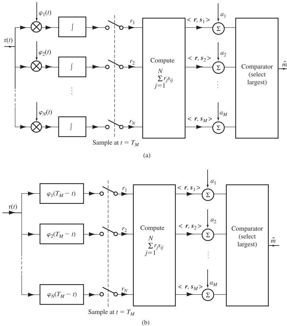
Figure 9.18 An alternative form of optimum M -ary receiver: (a) correlator; (b) matched filter.
