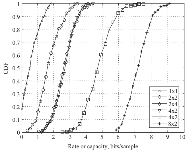
Figure 12.15 Cumulative distribution function (CDF) of different MIMO configurations.
