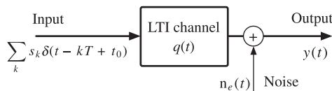
Figure 11.2 Baseband representation of QAM transmission over a linear time-invariant channel with ISI.
