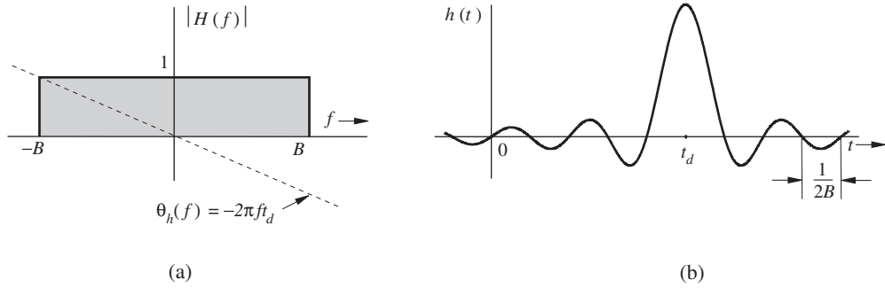
Figure 3.27 (a) Ideal lowpass filter frequency response and (b) its impulse response.
