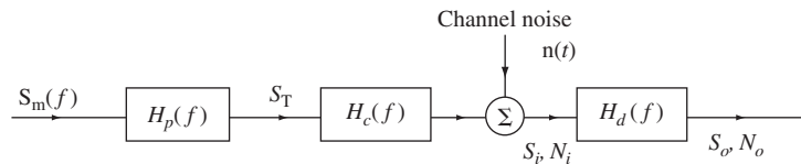
Figure 8.18 Optimum preemphasis and deemphasis filters in baseband systems.
