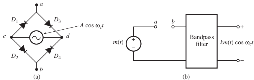
Figure 4.5 (a) Diode-bridge electronic switch. (b) Series-bridge diode modulator.
