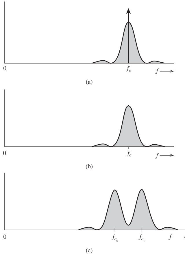
Figure 6.32 PSD of (a) ASK, (b) PSK, and (c) FSK.
