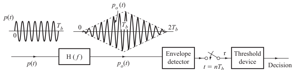
Figure 9.35 Noncoherent detection of digital modulated signals for ASK.
