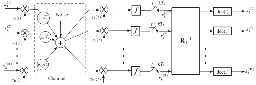
Figure 10.14 Decorrelator MUD receiver.
