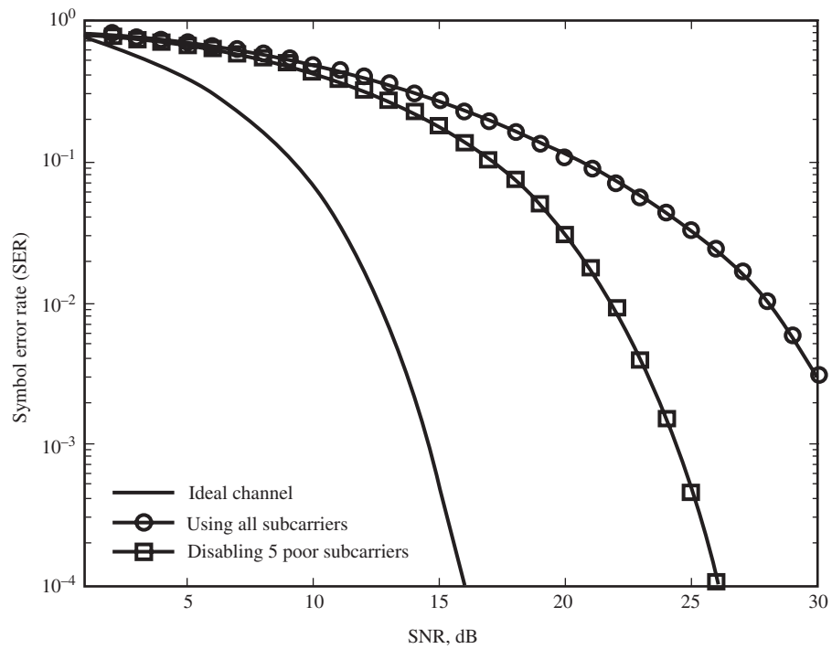
Figure 11.28 Average SER of the OFDM subcarriers before and after disabling five worst channels.
