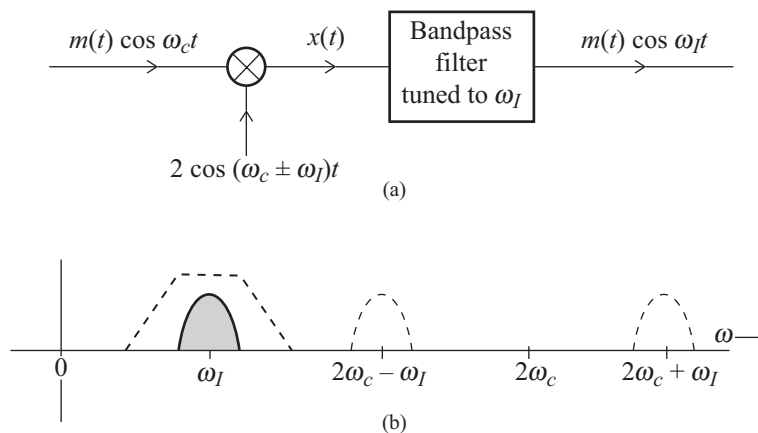
Figure 4.30 Frequency mixer or converter.
