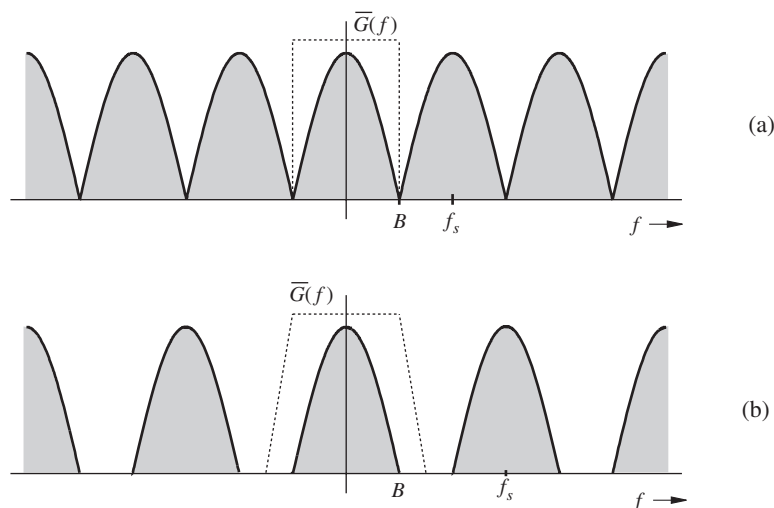
Figure 5.8 Spectra of a sampled signal: (a) at the Nyquist rate; (b) above the Nyquist rate.
