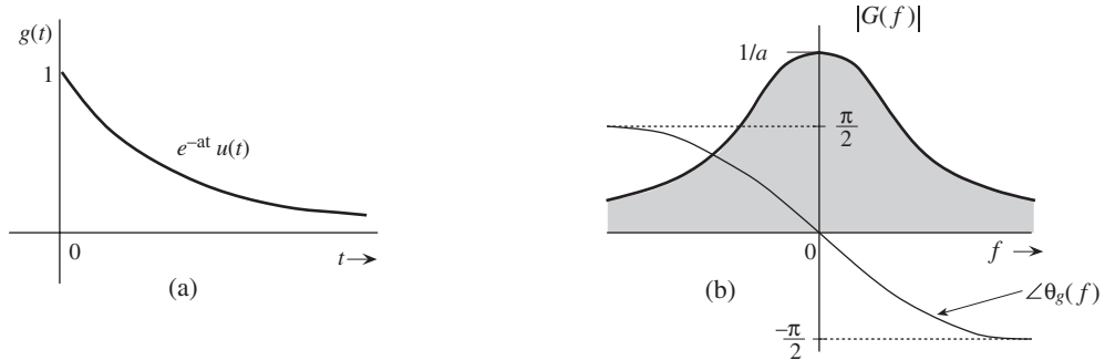
Figure 3.4 (a) e^{-at}u(t) and (b) its Fourier spectra.
