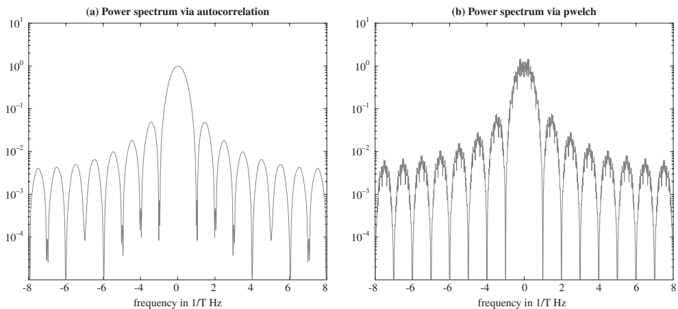
Figure 6.42 Power spectral densities of binary polar baseband modulation using the full-width rectangular NRZ pulse: (a) using autocorrelation method; (b) using Welch method of averaging periodograms.
