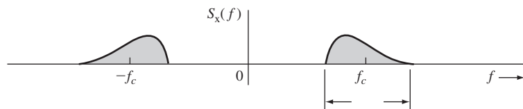
Figure 8.21 PSD of a bandpass random process.
