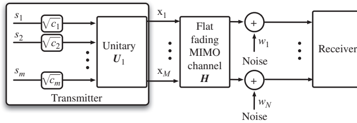
Figure 12.13 Water-pouring interpretation of the optimum MIMO transmission power loading based on channel knowledge.
