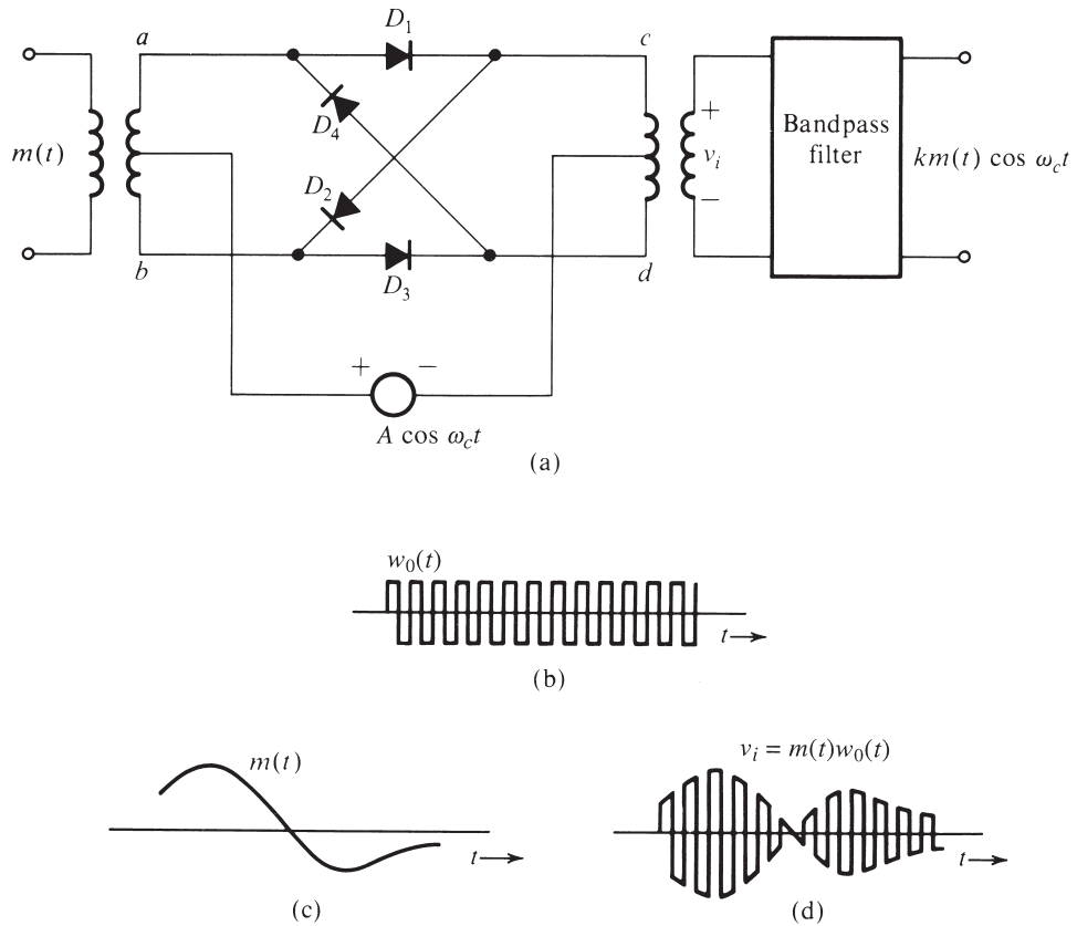
Figure 4.6 Ring modulation.
