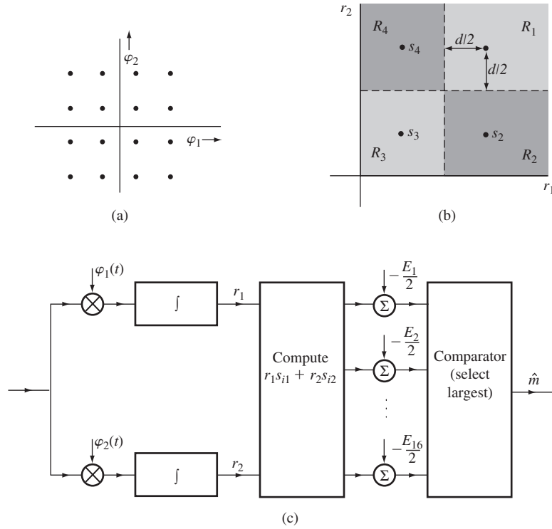
Figure 9.23 16-ary QAM.
