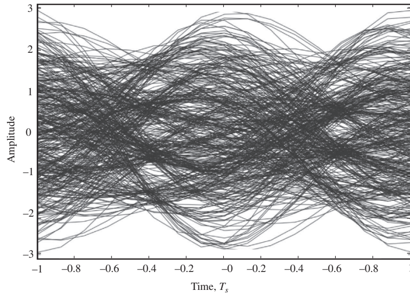
Figure 11.21 Noise-free eye diagram of the in-phase (real) component at the receiver (after matched filter) before sampling: the eyes are closed, and ISI will lead to decision errors.
