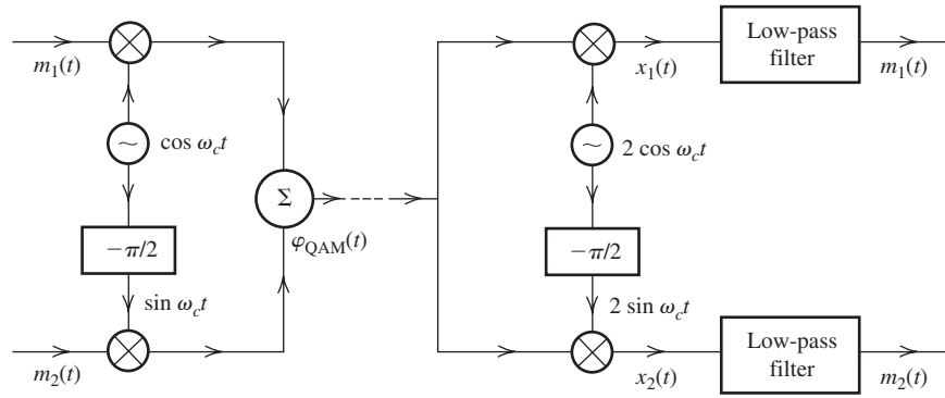
Figure 4.17 Quadrature amplitude modulation (QAM) and demodulation.
