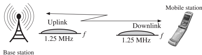
Figure 10.18 RF bandwidth requirements for IS-95 uplink and downlink.
