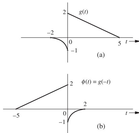
Figure 2.9 Time inversion (reflection) of a signal.
