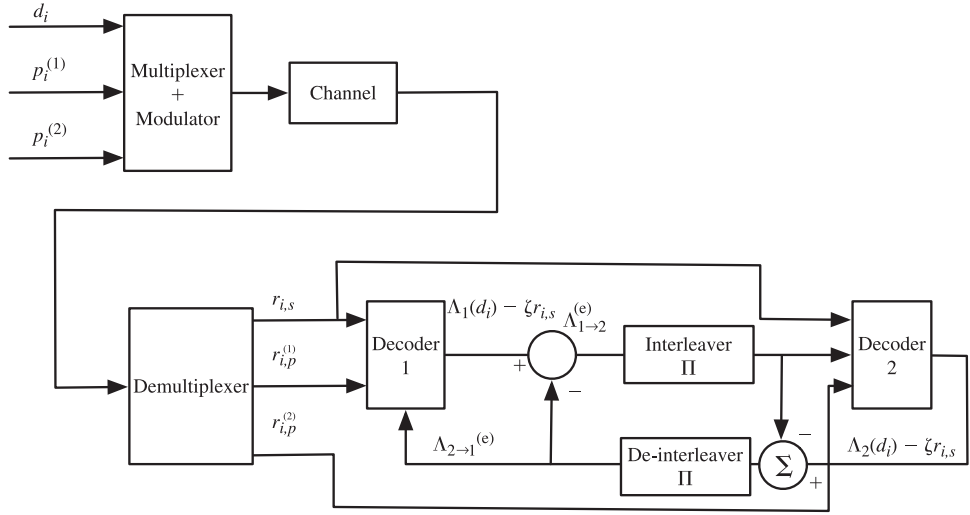
Figure 13.20 Exchange of extrinsic information between two component BCJR decoders for iterative turbo decoding.
