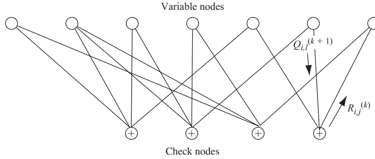
Figure 13.23 Message passing in the sum-product algorithm.
