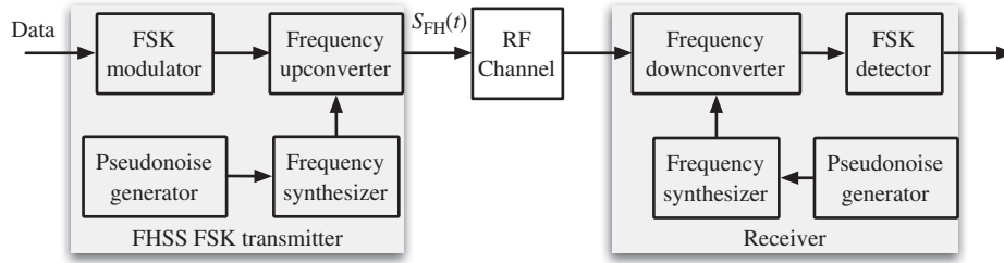
Figure 10.1 Frequency hopping spread spectrum system.
