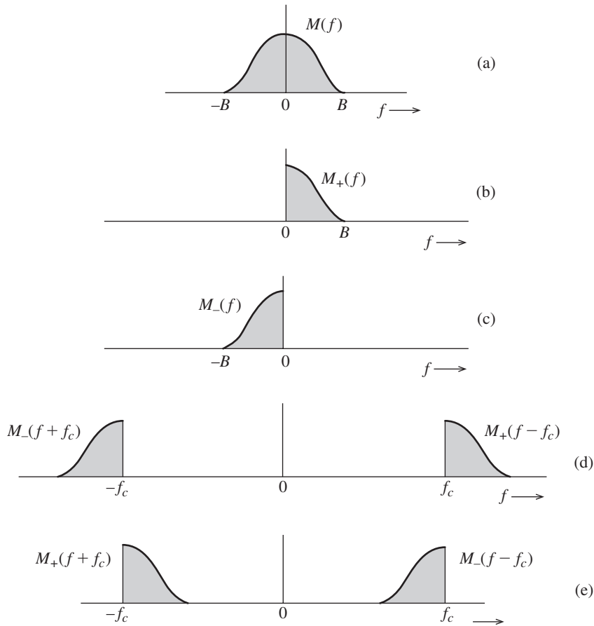
Figure 4.14 Expressing SSB spectra in terms of M_+(f) and M_-(f) .
