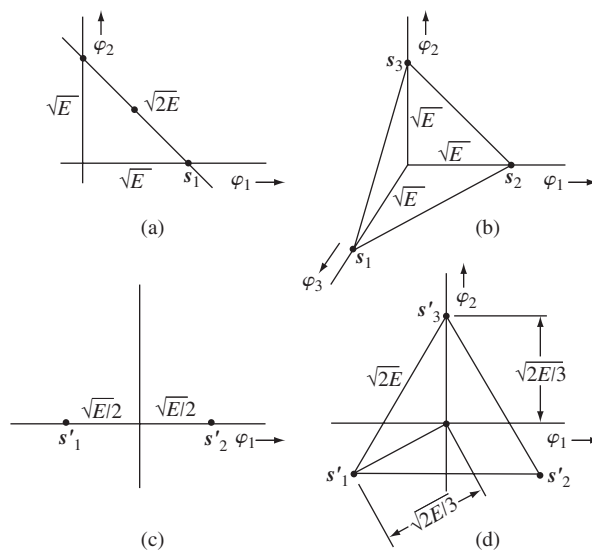
Figure 9.32 Simplex signals.
