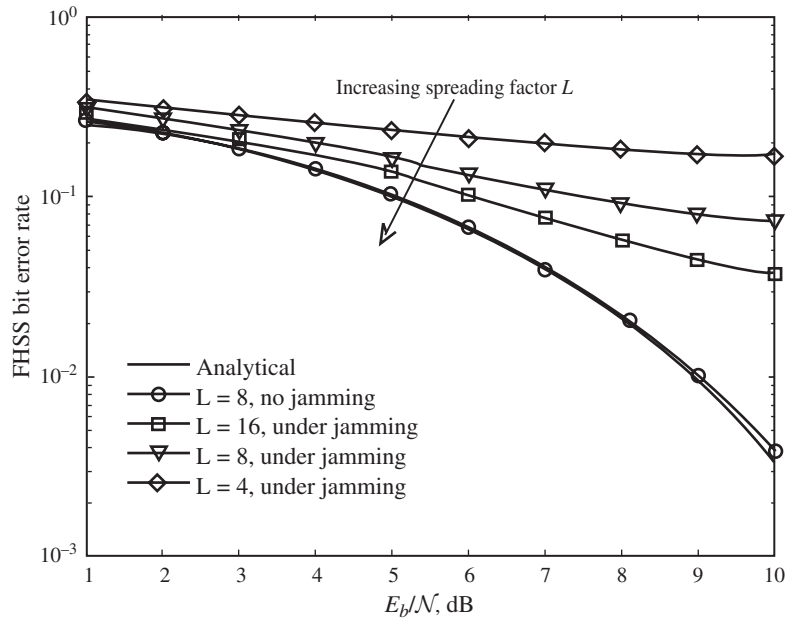
Figure 10.22 Performance of FHSS noncoherent detection under partial band jamming.
