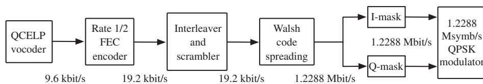
Figure 10.19 Forward link modulation and Walsh-Hadamard code spreading of cdmaOne (IS-95).
