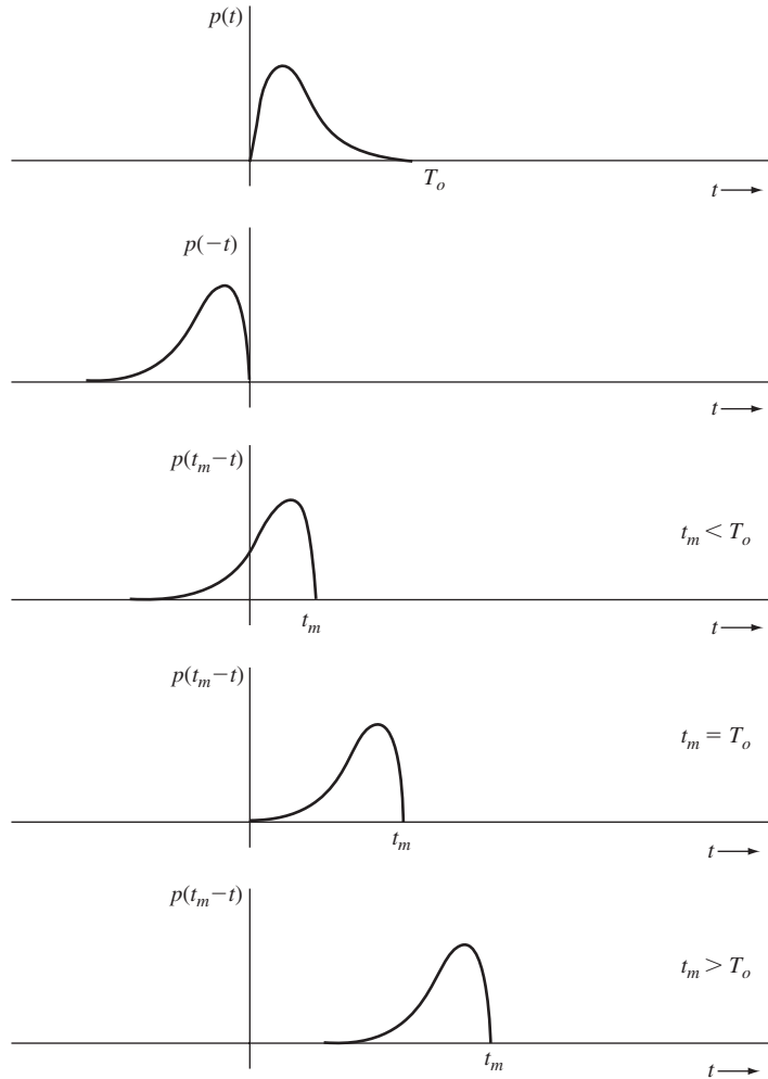
Figure 9.2 Optimum choice for sampling instant.
