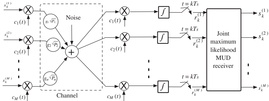
Figure 10.13 Maximum likelihood multiuser detection (MUD) receiver.
