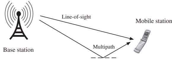
Figure 11.1 Simple illustration of a two-ray multipath channel.
