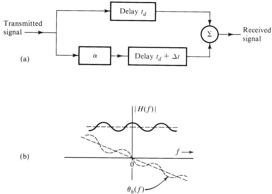
Figure 3.35 Multipath transmission.
