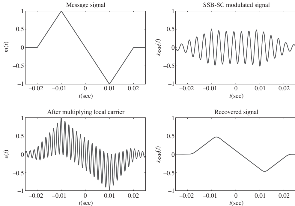
Figure 4.46 Time domain signals during SSB-SC modula- tion and coherent demodulation.
