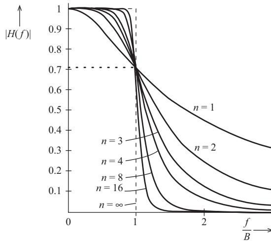
Figure 3.30 Butterworth filter characteristics.
