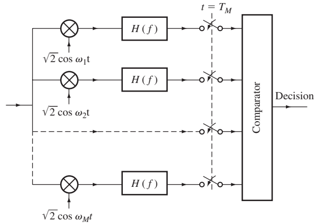
Figure 9.28 Coherent MFSK receiver.
