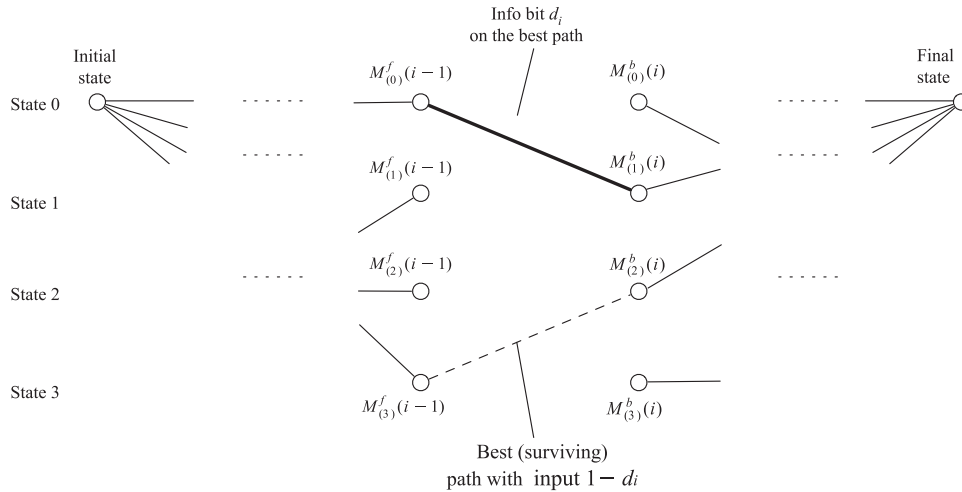
Figure 13.18 Trellis diagram of soft output Viterbi algorithm (SOVA).
