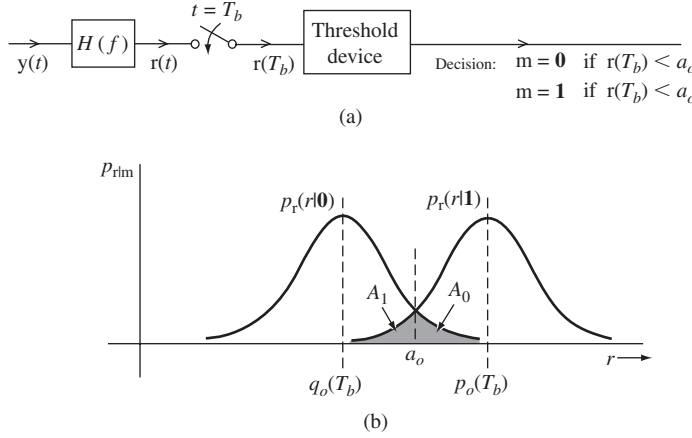
Figure 9.4 Optimum binary threshold detection.
