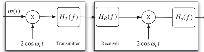
Figure 4.21 Transmitter filter H_T(f) , receiver front-end filter H_R(f) , and the receiver output lowpass filter H_o(f) in VSB television systems.
