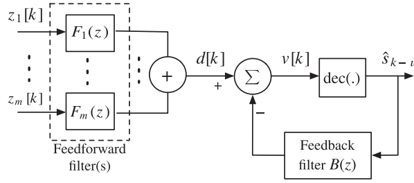
Figure 11.8 A decision feedback equalizer with fractionally spaced samples.
