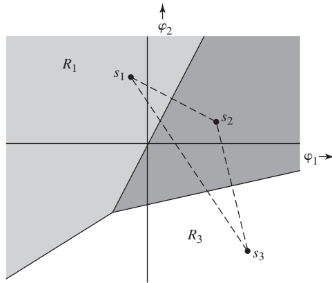
Figure 9.20 Determining optimum decision regions.
