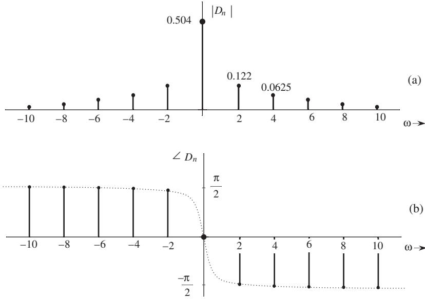
Figure 2.23 Exponential Fourier spectra for the signal in Fig. 2.19a.
