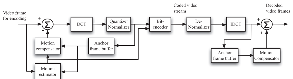
Figure 5.37 MPEG-2 video encoding system.
