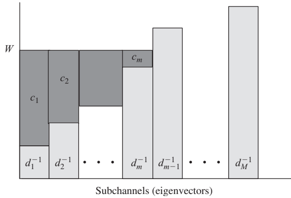
Figure 12.12 Water-filling interpretation of MIMO transmission power loading based on channel knowledge.
