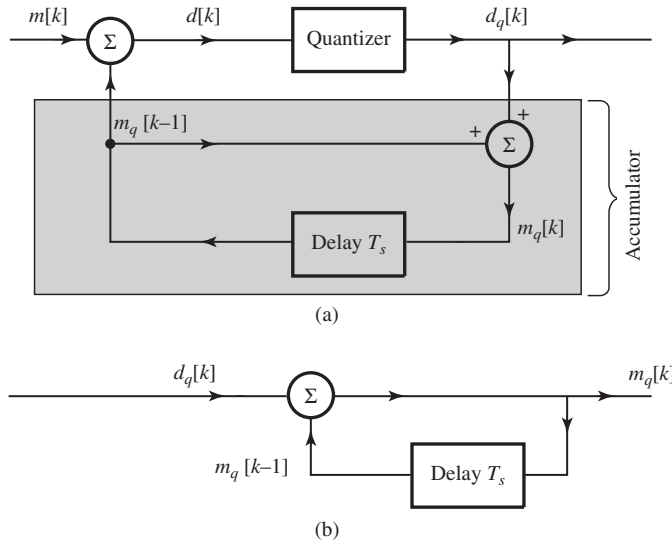
Figure 5.31 Delta modulation is a special case of DPCM.
