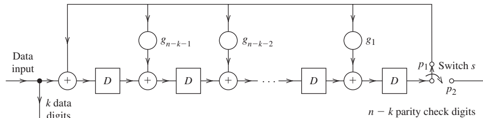
Figure 13.2 Encoder for systematic cyclic code.
