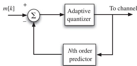
Figure 5.30 ADPCM encoder uses an adaptive quantizer controlled only by the encoder output bits.
