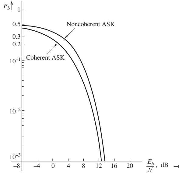
Figure 9.37 Error probability of noncoherent ASK detection.
