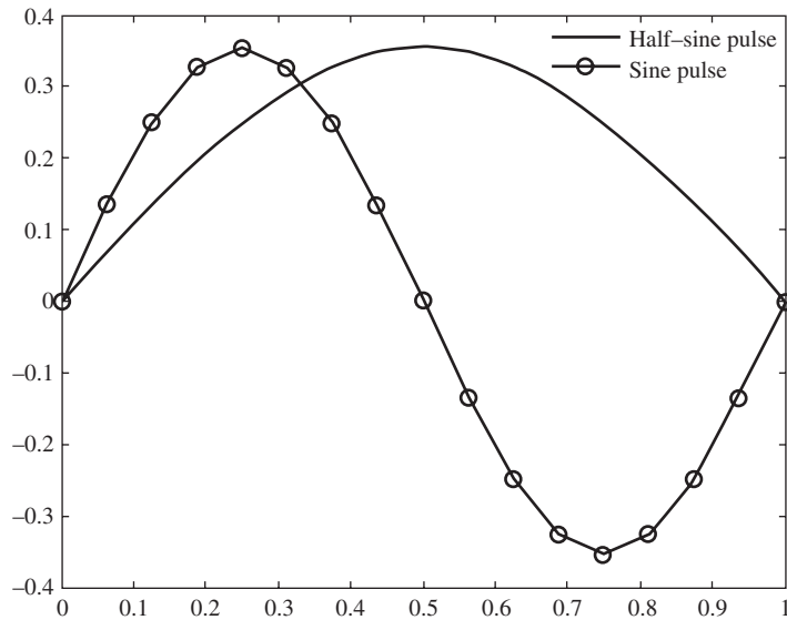
Figure 9.45 Waveforms of the two pulses used in orthogonal binary signaling: solid curve, half-sine pulse; curve with circles, sine pulse.
