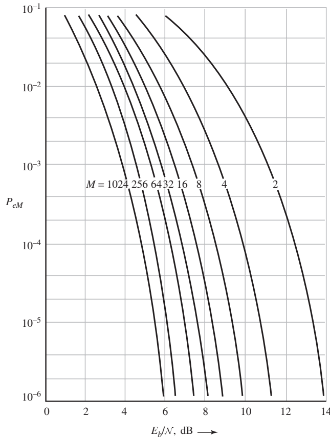
Figure 9.39 Error probability of noncoherent MFSK.
