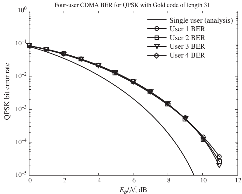
Figure 10.25 Performance of DS-CDMA conventional single-user detection without the near-far effect.
