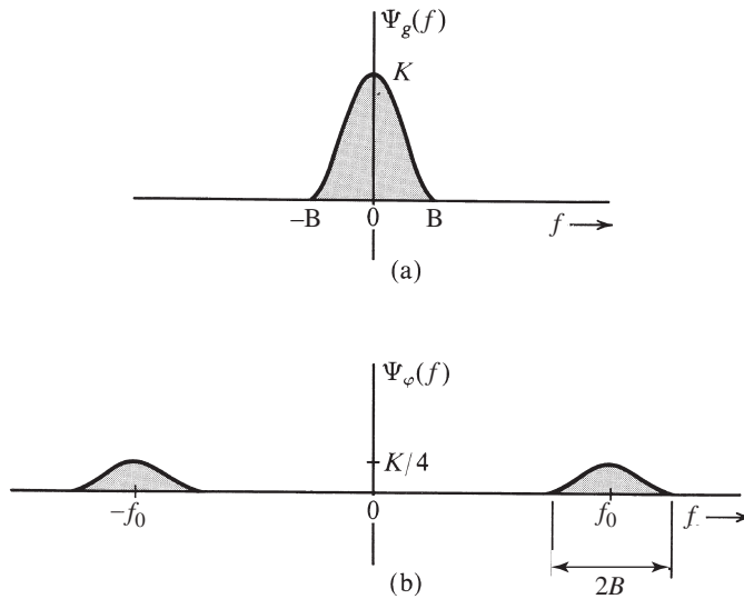
Figure 3.39 Energy spectral densities of (a) modulating and (b) modulated signals.
