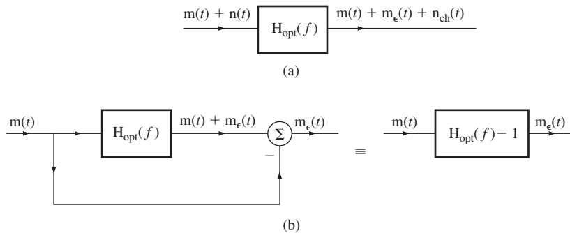
Figure 8.15 Wiener-Hopf filter operation.
