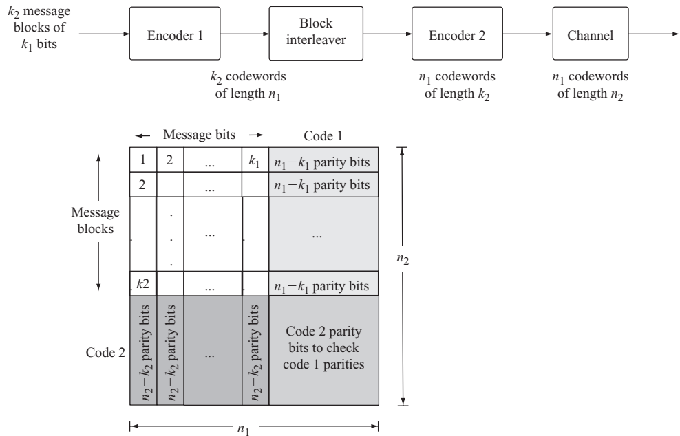
Figure 13.15 Product code formed by two encoders separated by a block interleaver.
