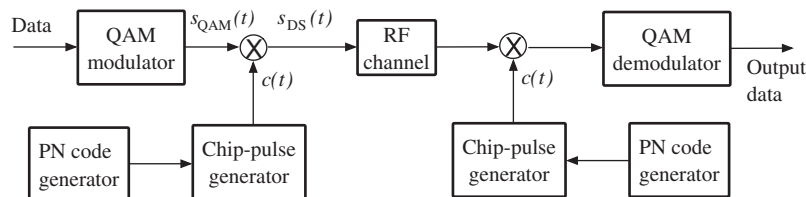
Figure 10.8 DSSS system.
