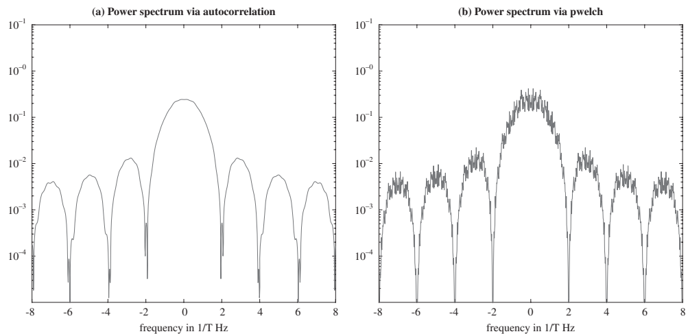
Figure 6.41 Power spectral densities of binary polar baseband modulation using the half-width rectangular RZ pulse: (a) using autocorrelation method; (b) using Welch method of averaging periodograms.
