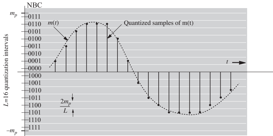
Figure 5.15 Quantization of analog signal samples.
