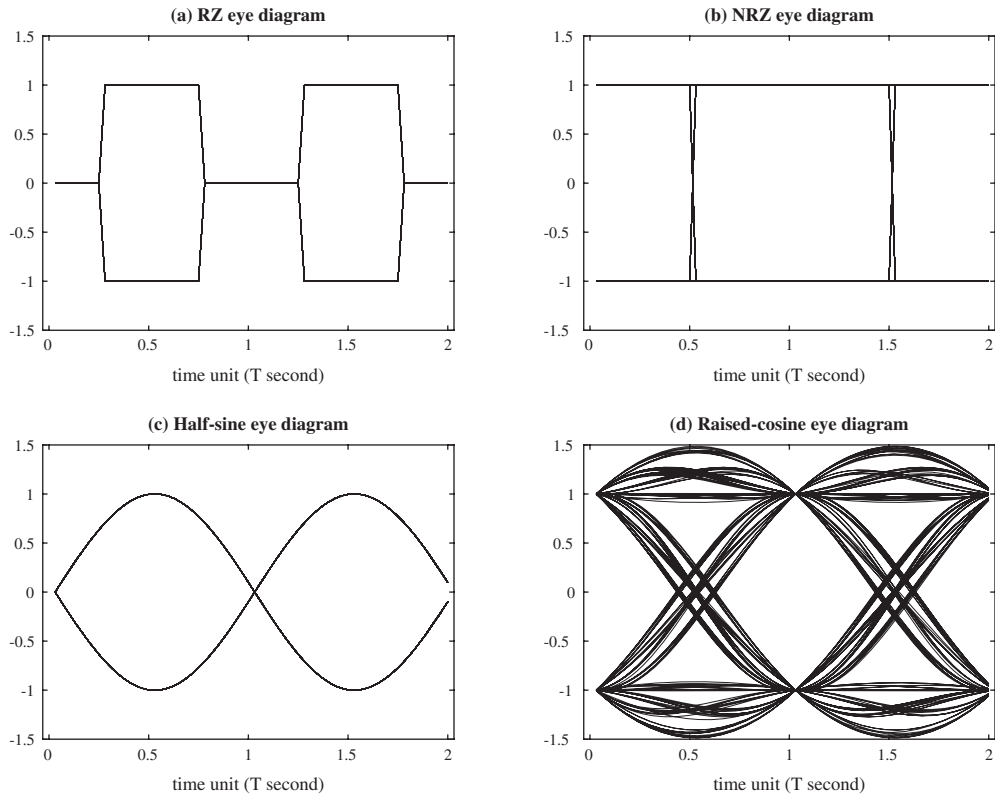
Figure 6.40 Eye diagrams of binary polar baseband modulation waveforms using (a) Half-width rectangular RZ pulse; (b) Rectangular NRZ pulse with half-symbol offset; (c) Half-sine pulse; (d) Raised cosine pulse with rolloff factor of 0.5.
