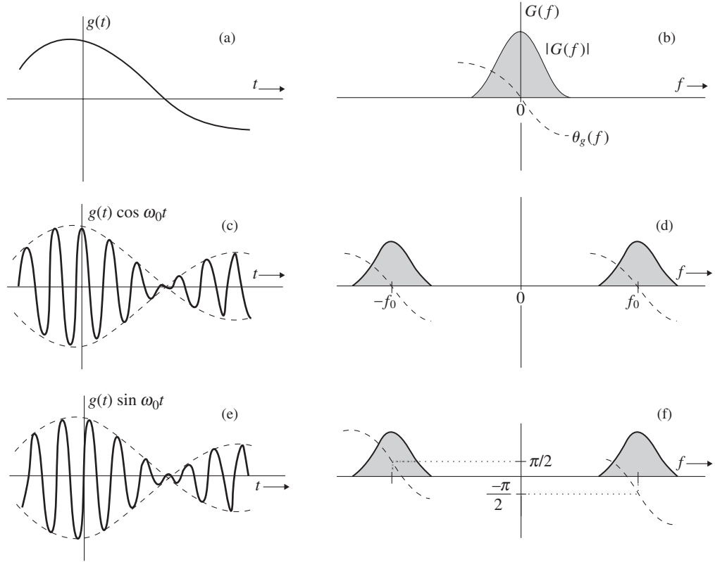
Figure 3.19 Amplitude modulation of a signal causes spectral shifting.
