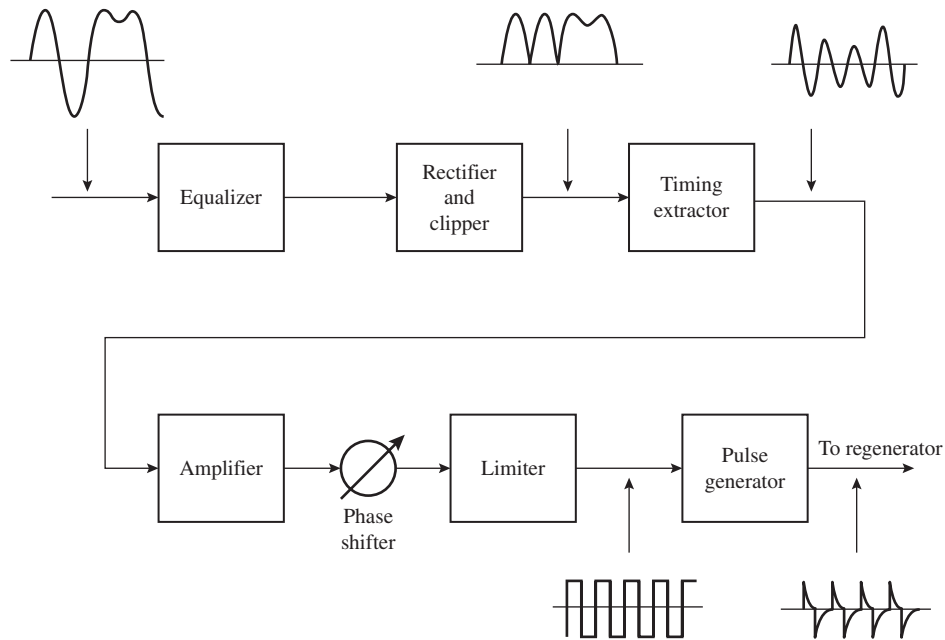
Figure 6.23 Timing extraction.
