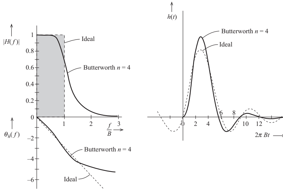
Figure 3.31 Comparison of Butterworth filter ( n = 4 ) and an ideal filter.
