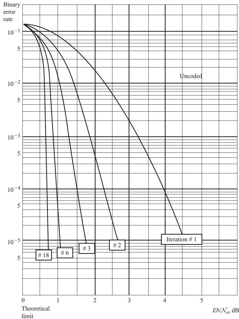
Figure 13.21 Decoding performance of a rate 1/2 Turbo code is shown to be very close to the theoretical limit. (©2017 IEEE. Reprinted, with permission, from C. Berrou and A. Glavieux, "Near Optimum Error Correcting Coding and Decoding: Turbo-Codes," IEEE Trans. Commun., vol. 44, no. 10, pp. 1261–1271, October 1996.)
