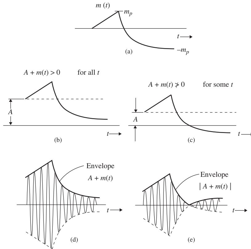
Figure 4.7 AM signal and its envelope.
