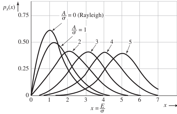
Figure 8.28 Ricean PDF.
