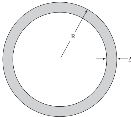
Figure 12.7 Volume of a shell of a D -dimensional hypersphere.
