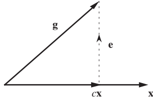
Figure 2.13 Component (projection) of a vector along another vector.
