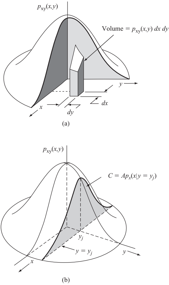
Figure 7.13 (a) Joint PDF. (b) Conditional PDF.
