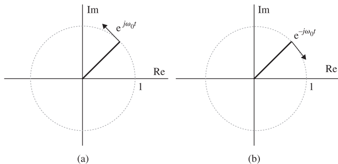
Figure 2.24 (a) Unit length complex variable with positive frequency (rotating counterclockwise) and (b) unit length complex variable with negative frequency (rotating clockwise).
