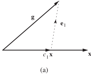
Figure 2.14 Approximations of a vector in terms of another vector.
