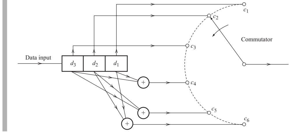
Figure 13.1 Encoder for linear block codes.
