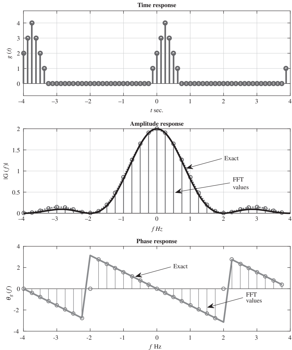
Figure 3.48 Fourier transform of a delayed triangle pulse \Delta(t - 2T_s) .
