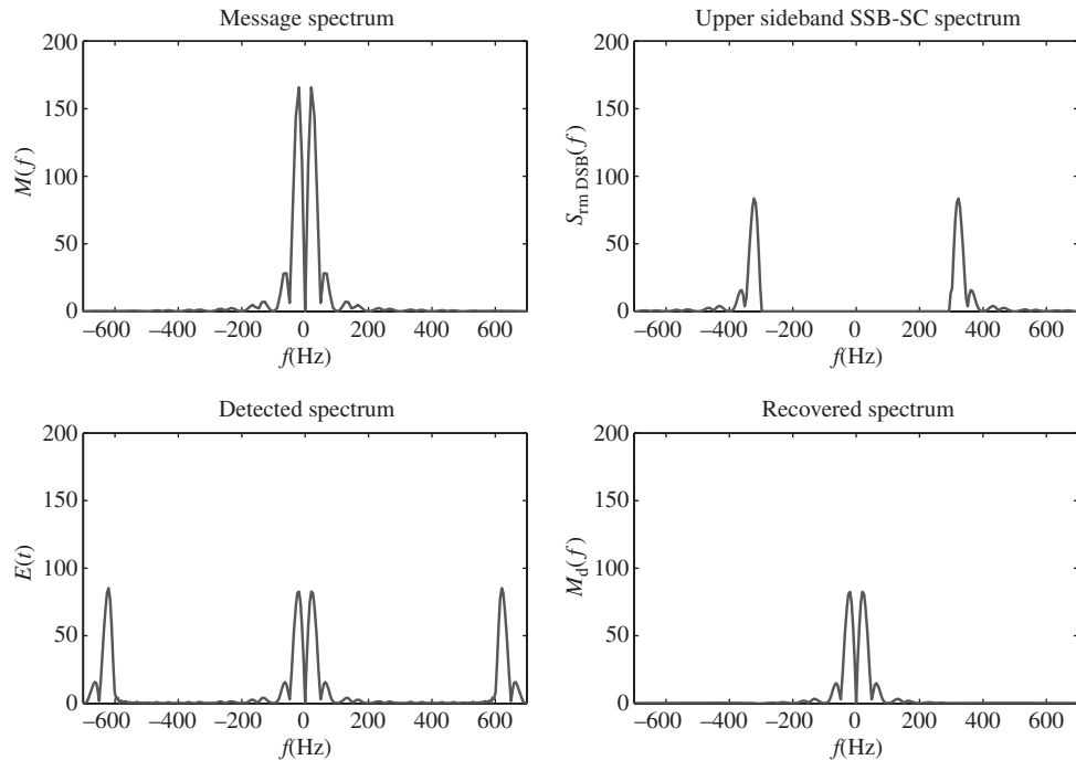
Figure 4.47 Frequency domain signals in SSB-SC modulation and coherent demodulation.
