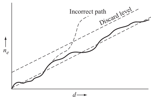
Figure 13.12 Setting the threshold in sequential decoding.
