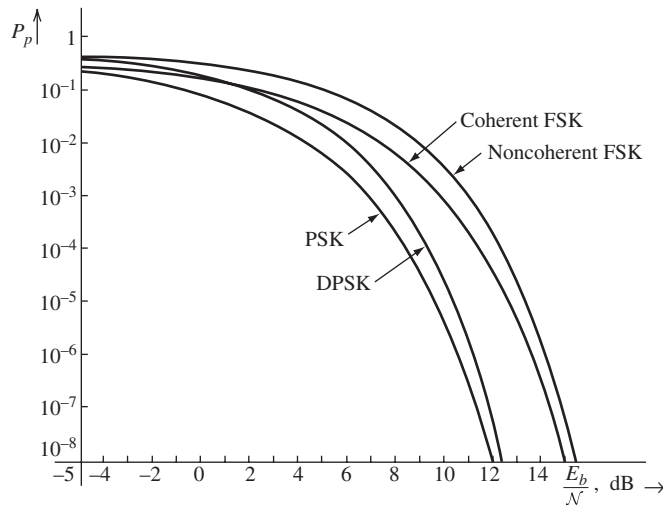
Figure 9.41 Error probability of PSK, DPSK, and coherent and noncoherent FSK.
