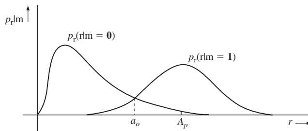
Figure 9.36 Conditional PDFs in the noncoherent detection of ASK signals.
