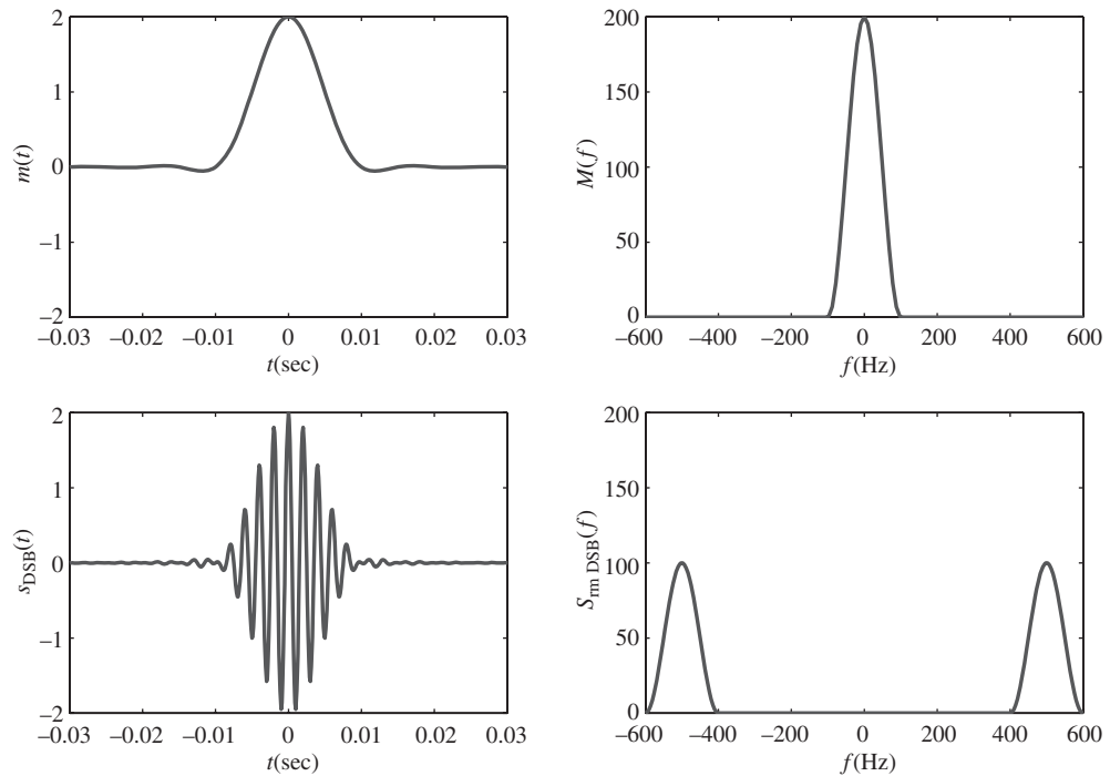
Figure 4.41 Example signals in time and frequency domains during DSB-SC modulation.
