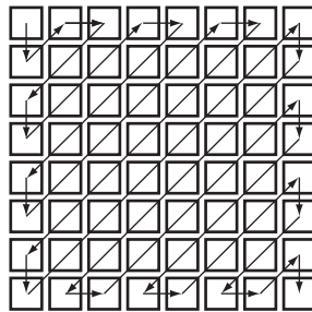
Figure 5.39 Zigzag DCT coefficient scanning pattern.
