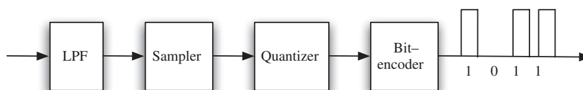
Figure 5.14 PCM system diagram.
