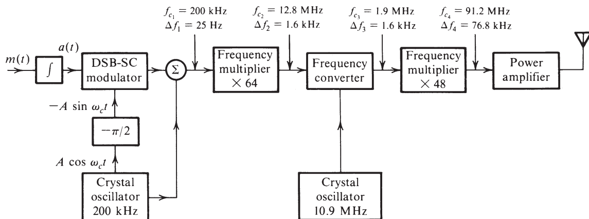
Figure 4.33 Block diagram of the Armstrong indirect FM transmitter.
