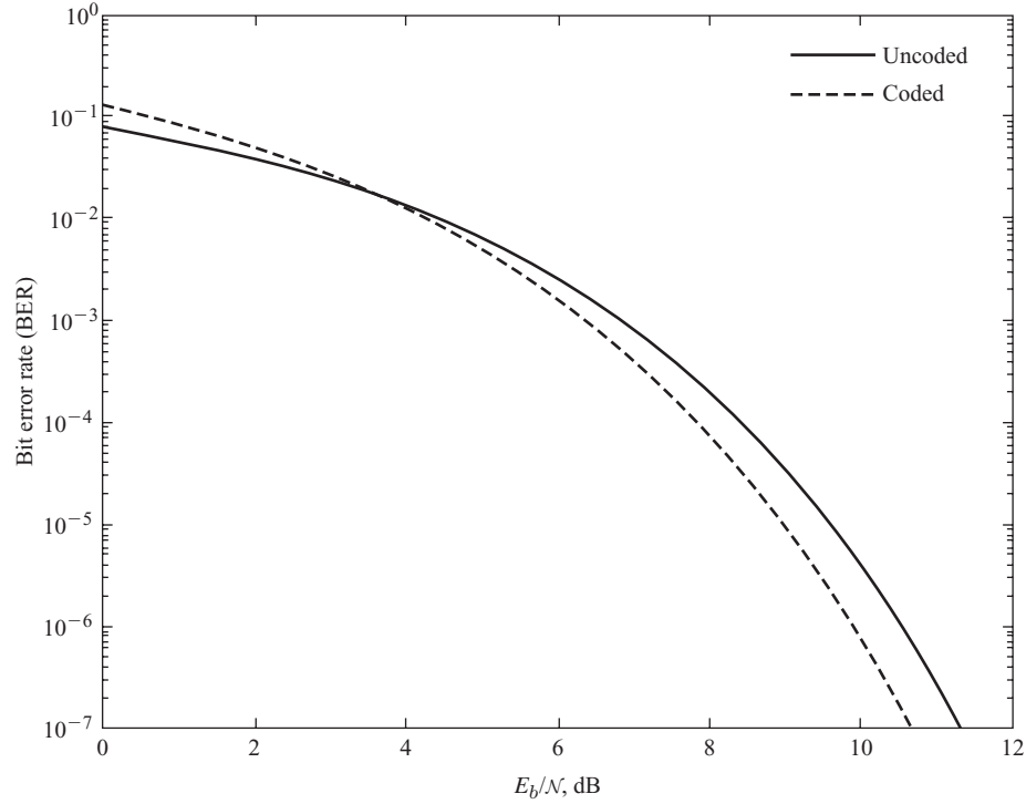
Figure 13.3 Performance comparison of coded (dashed) and uncoded (solid) systems.
