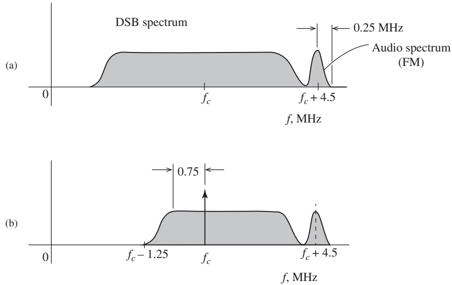
Figure 4.22 NTSC analog television signal spectra: (a) DSB video signal plus audio; (b) signal transmitted.
