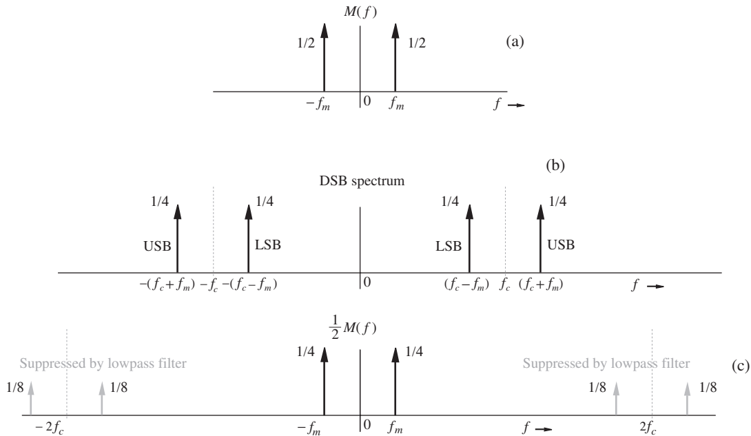
Figure 4.2 Example of DSB-SC modulation.
