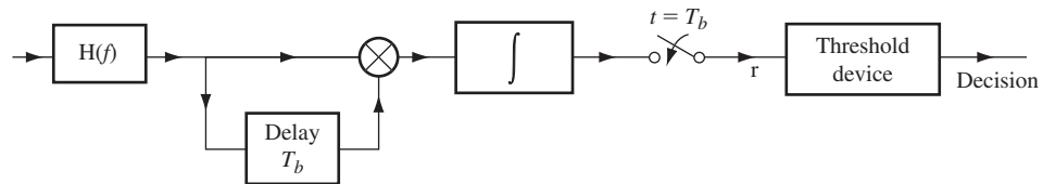
Figure 9.40 Differential binary PSK detection.
