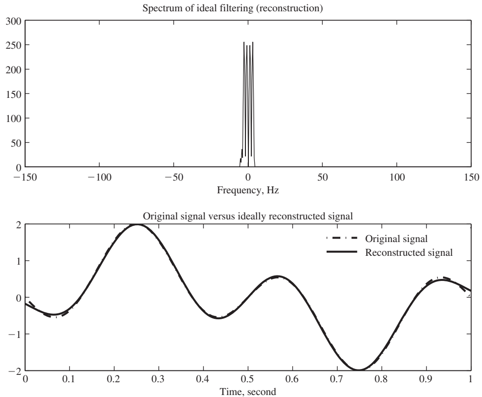
Figure 5.42 Reconstructed signal spectrum and waveform from applying the ideal impulse sampling and ideal LPF recon- struction.
