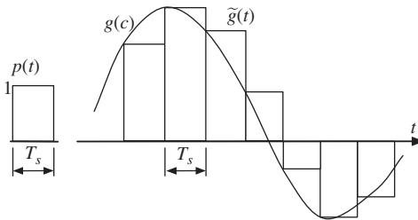
Figure 5.7 Practical signal reconstruction using flat-top (rectangular) pulses of duration T_s .
