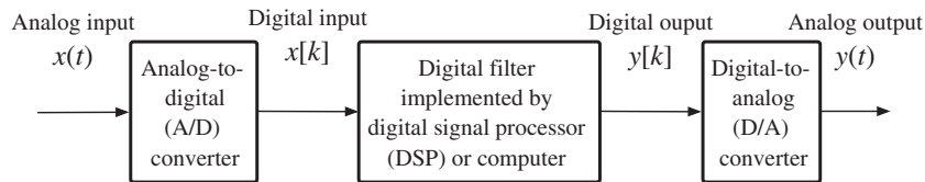
Figure 3.32 Basic diagram of a digital filter in practical applications.
