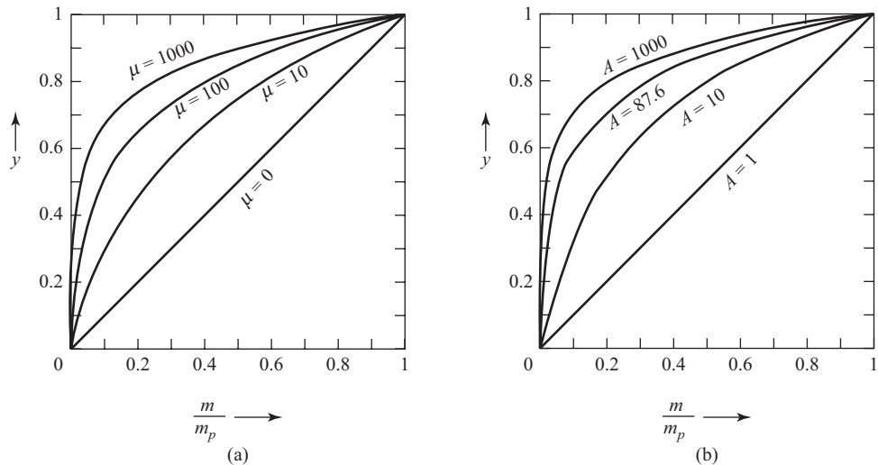
Figure 5.17 (a) \mu -law characteristic. (b) A -law characteristic.
