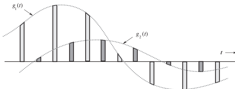
Figure 5.13 Time division multiplexing of two signals.
