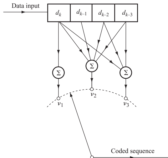
Figure 13.10 Convolutional encoder.
