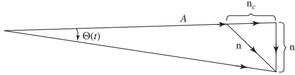
Figure 8.27 Phasor representation of a sinusoid and a narrowband Gaussian noise.
