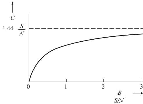
Figure 12.5 Channel capacity versus bandwidth for a channel with white Gaussian noise and fixed signal power.
