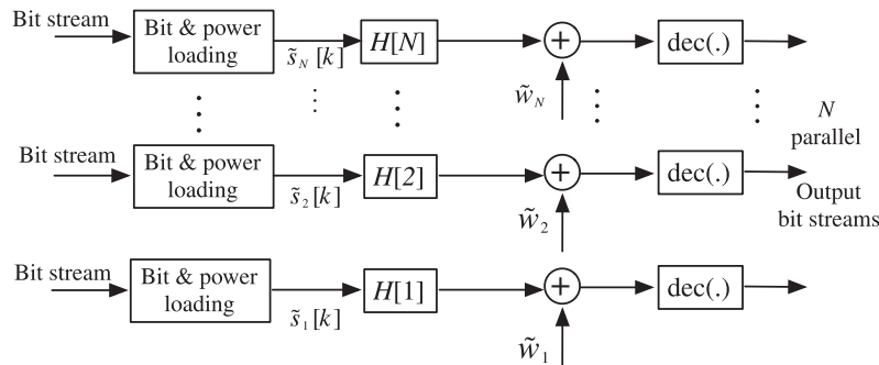
Figure 11.14 Bit and power loading in a DMT (OFDM) transmission system with N subcarriers.
