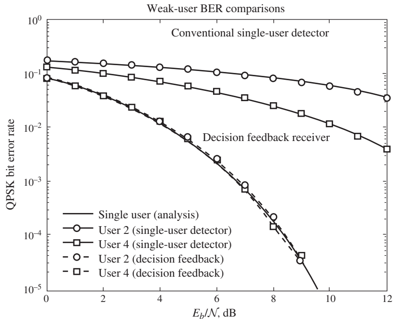
Figure 10.27 Performance of decision feedback MUD in comparison with the conventional single-user receiver.
