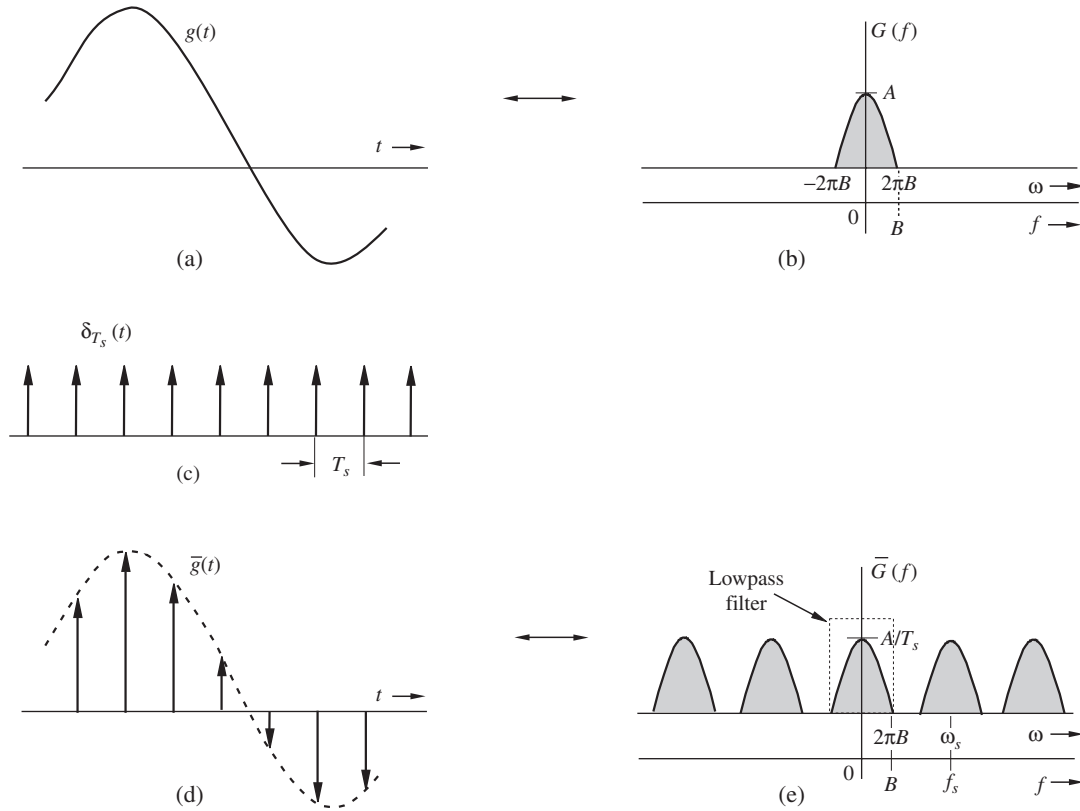
Figure 5.1 Sampled signal and its Fourier spectra.
