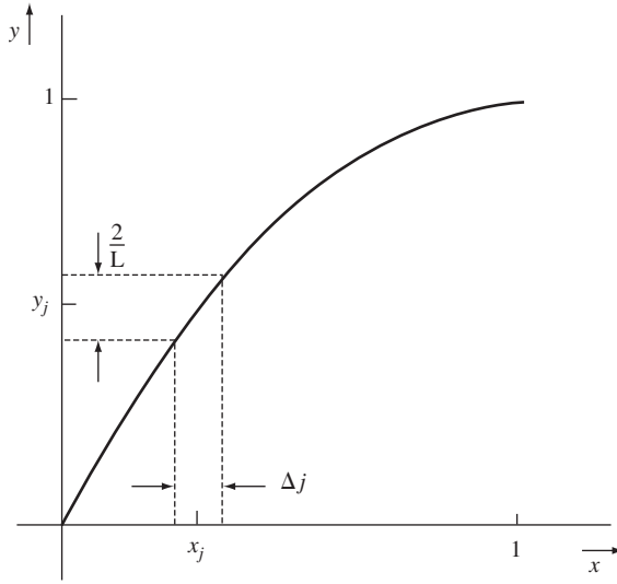
Figure 8.19 Input-output characteristic of a PCM compressor.
