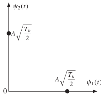
Figure 6.36 Binary FSK symbols in the two-dimensional orthogonal signal space.
