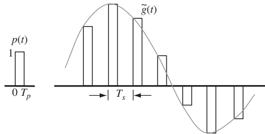
Figure 5.6 Simple interpolation by means of simple rectangular pulses.
