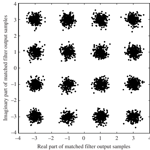
Figure 9.49 Scatter plot of the matched filter output for the 16-QAM signaling with root-raised cosine pulse when E_b/\mathcal{N} = 18 dB.
