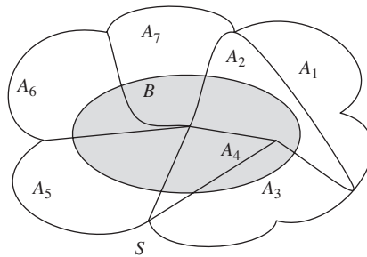
Figure 7.4 The event of interest B and the partition of S by \{A_i\} .
