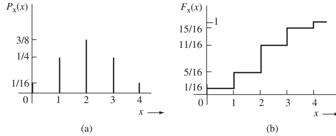
Figure 7.8 (a) Probabilities P_x(x_i) and (b) the cumulative distribution function (CDF).
