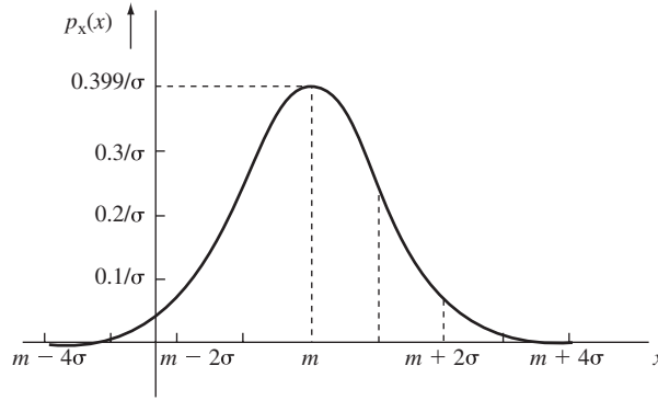
Figure 7.11 Gaussian PDF with mean m and variance \sigma^2 .
