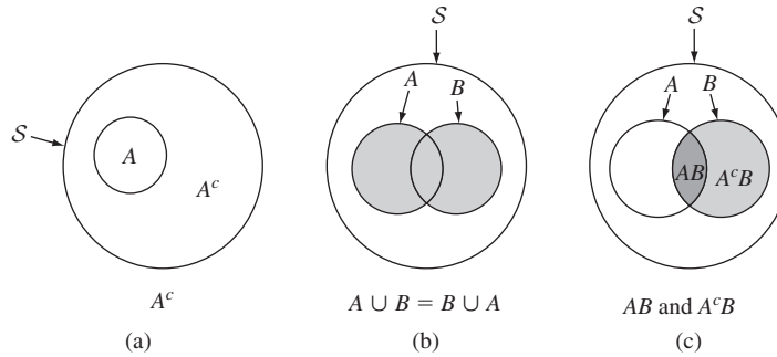
Figure 7.2 Representation of (a) complement, (b) union, and (c) intersection of events.
