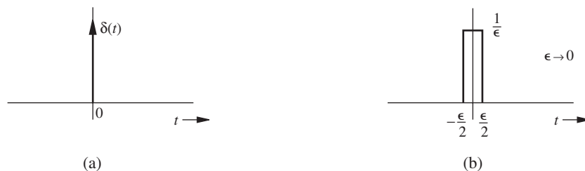
Figure 2.11 (a) Unit impulse and (b) its approximation.
