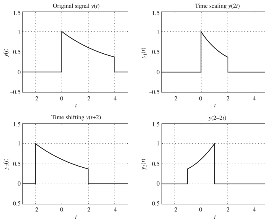
Figure 2.28 Examples of basic signal operations.
