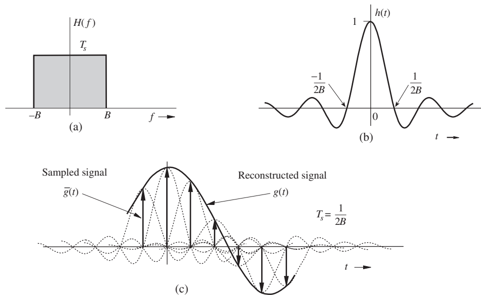
Figure 5.2 Ideal signal reconstruction through interpolation.
