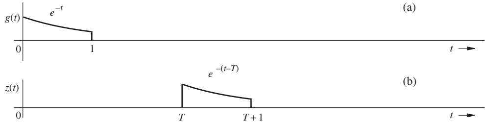
Figure 2.17 Explanation of the need for correlation function.
