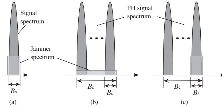
Figure 10.3 Effects of (a) narrowband jamming, (b) FHSS under broadband jamming, and (c) partial band jamming.
