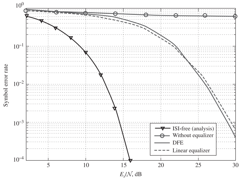
Figure 11.24 Symbol error rate (SER) comparison of DFE, linear equalization, and under ideal channel.
