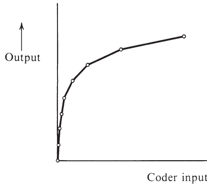
Figure 5.20 Piecewise linear compressor characteristic.
