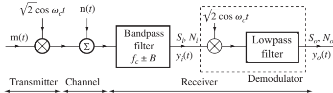
Figure 8.30 DSB-SC system.
