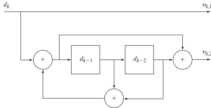
Figure 13.8 A recursive systematic convolutional (RSC) encoder.
