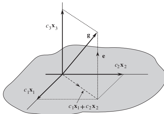
Figure 2.18 Representation of a vector in three-dimensional space.
