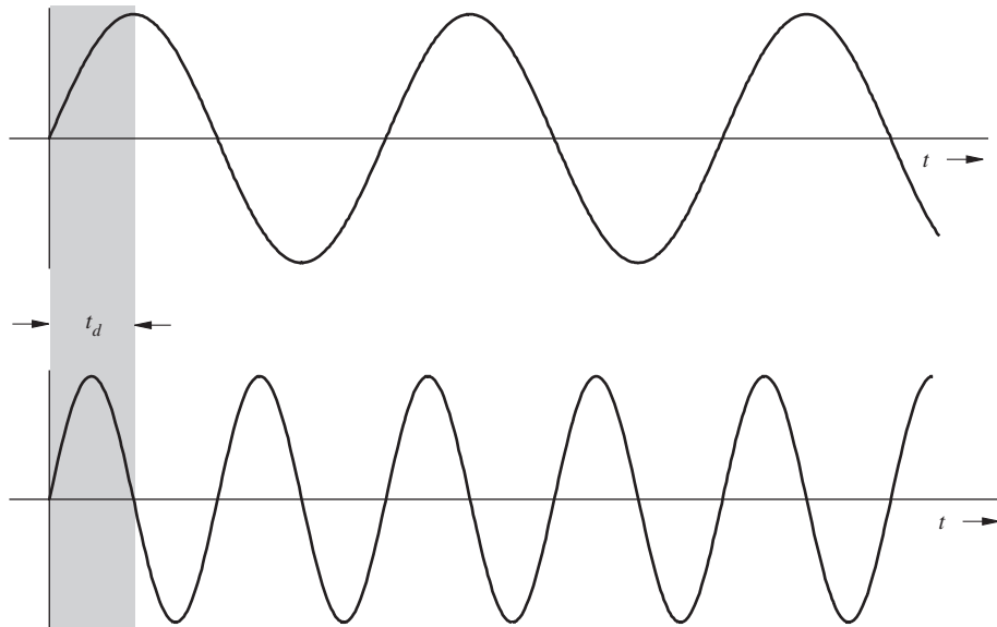
Figure 3.17 Physical explanation of the time-shifting property.
