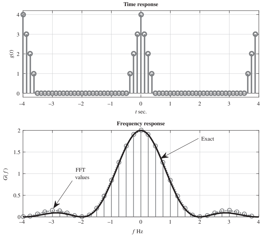
Figure 3.47 Discrete Fourier transform of a triangular pulse.
