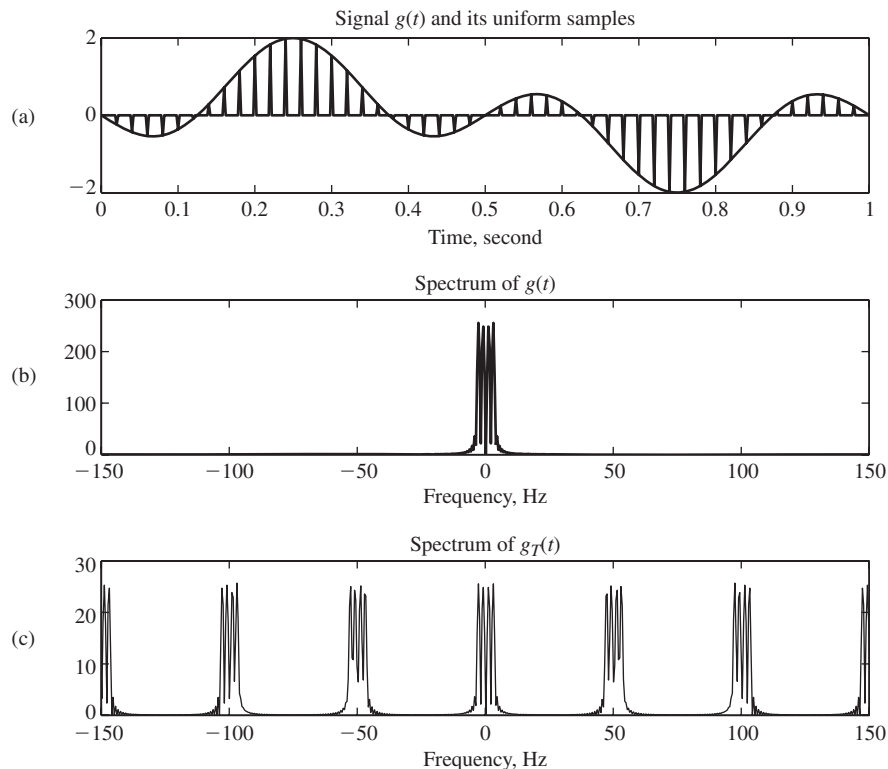
Figure 5.41 The relationship between the original signal and the ideal uniformly sampled signal in the time (a) and frequency (b, c) domains.
