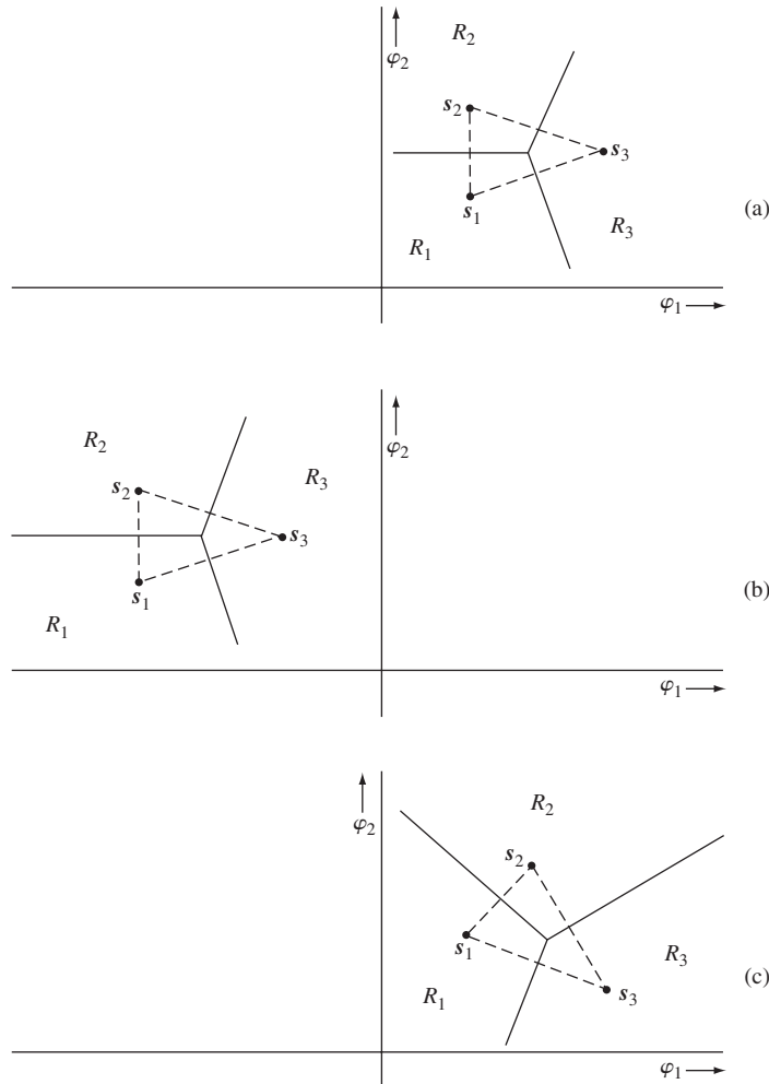
Figure 9.29 Translation and rotation of coordinate axes.
