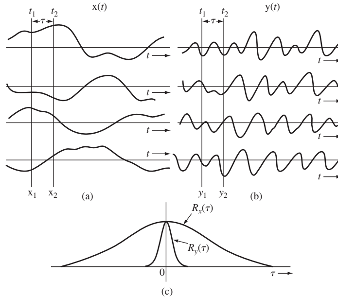
Figure 8.4 Autocorrelation functions for a slowly varying and a rapidly varying random process.
