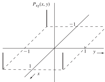
Figure 7.6 Representation of joint probabilities of two random variables.
