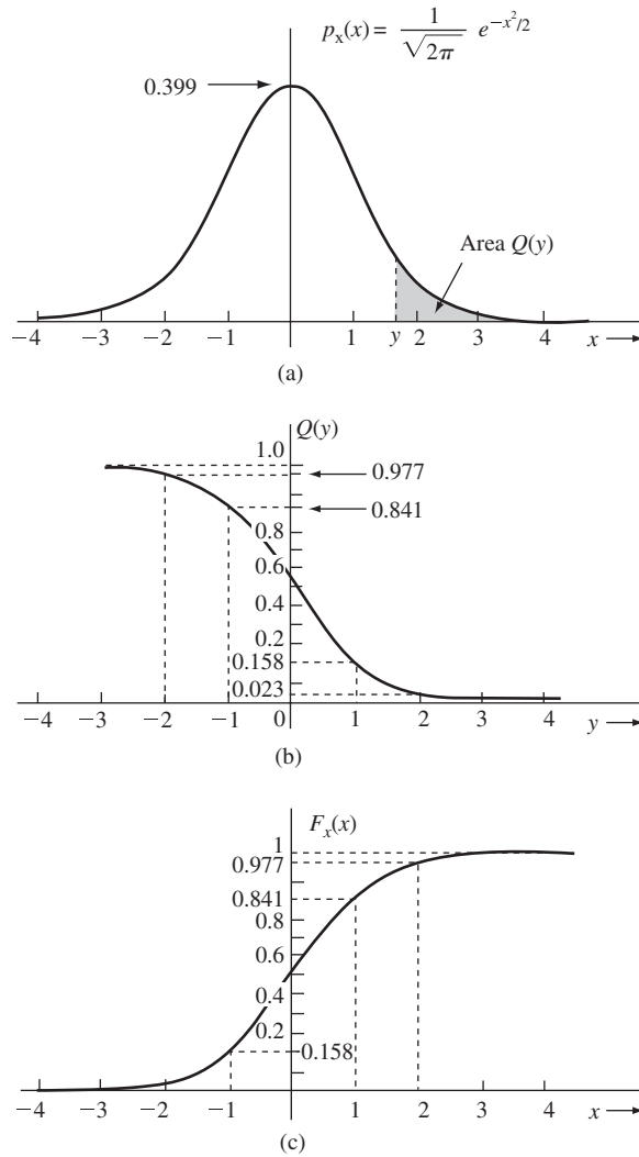
Figure 7.10 (a) Gaussian PDF. (b) Function Q(y) . (c) CDF of the Gaussian PDF.
