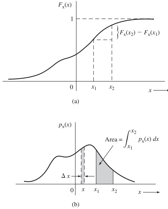
Figure 7.9 (a) Cumulative distribution function (CDF). (b) Probability density function (PDF).
