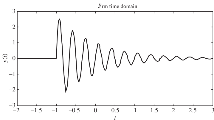
Figure 2.27 Graphing a signal.
