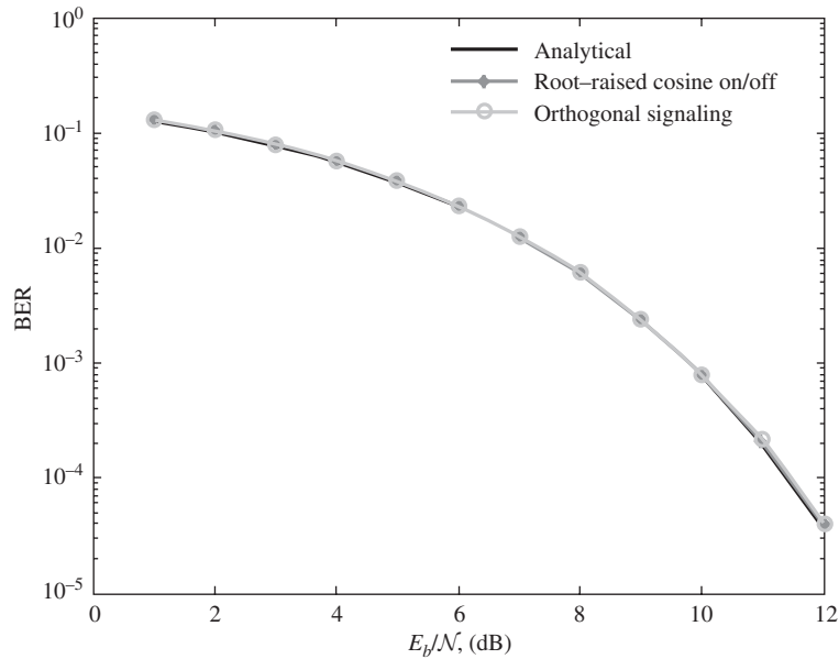
Figure 9.46 Measured BER results in comparison with analytical BER.
