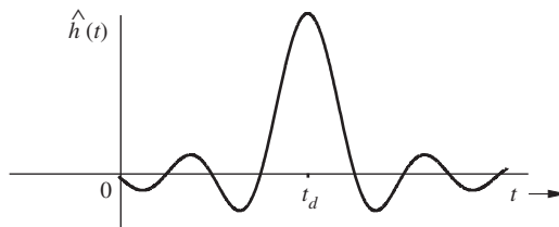
Figure 3.29 Approximate realization of an ideal lowpass filter by truncating its impulse response.
