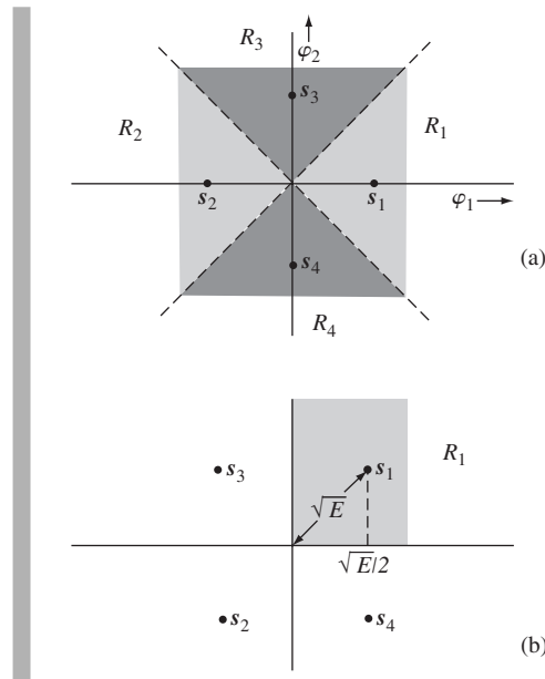
Figure 9.30 Analysis of QPSK.
