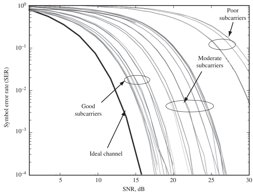
Figure 11.27 Symbol error rate (SER) of all 32 subcarriers over the multipath channel.
