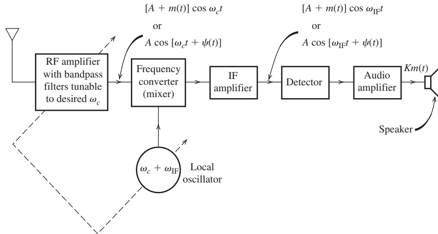
Figure 4.31 Superheterodyne receiver.
