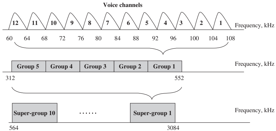
Figure 4.35 Analog L -carrier hierarchical frequency division multiplexing for long-haul telephone systems.
