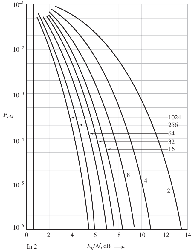
Figure 9.27 Error probability of orthogonal signaling and coherent MFSK.
