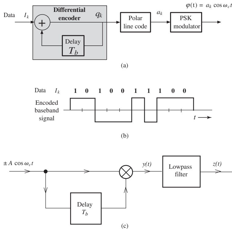
Figure 6.35 (a) Differential encoding; (b) encoded signal; (c) differential PSK receiver.
