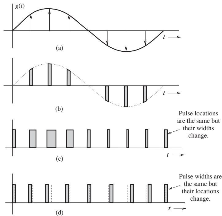
Figure 5.12 Pulse-modulated signals. (a) The unmodulated signal. (b) The PAM signal. (c) The PWM signal. (d) The PPM signal.
