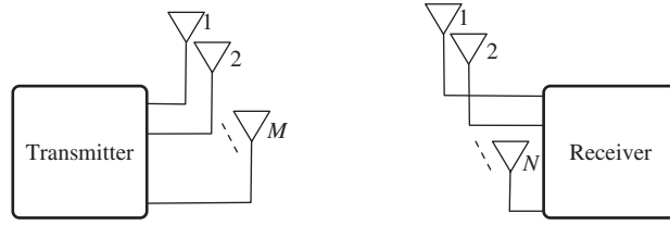
Figure 12.10 MIMO system with M transmit antennas and N receive antennas.
