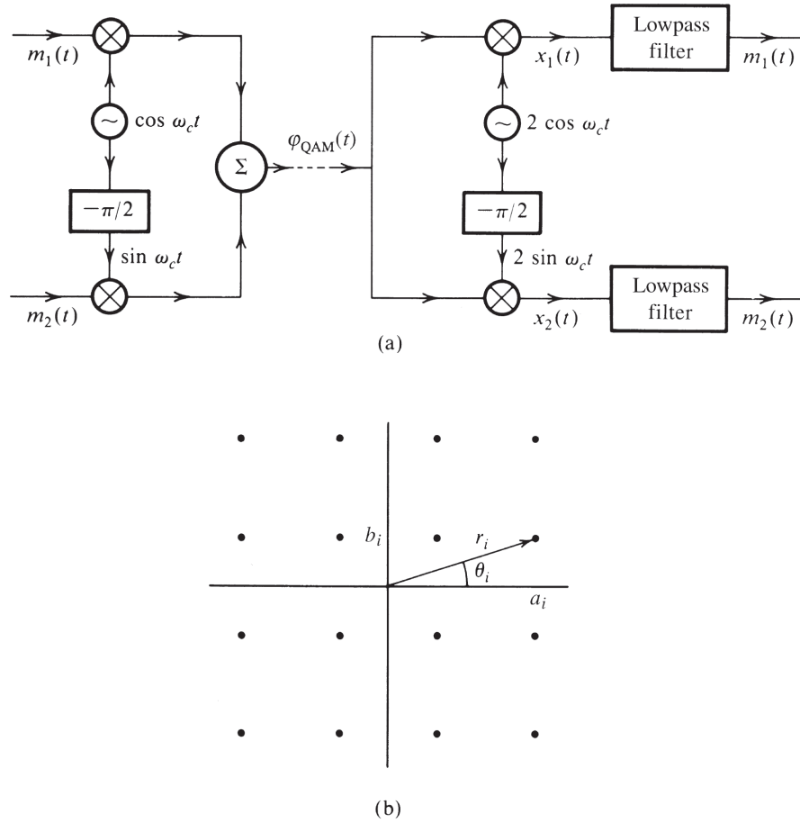
Figure 6.38 (a) QAM or quadrature multiplexing and (b) 16-point QAM ( M = 16 ).
