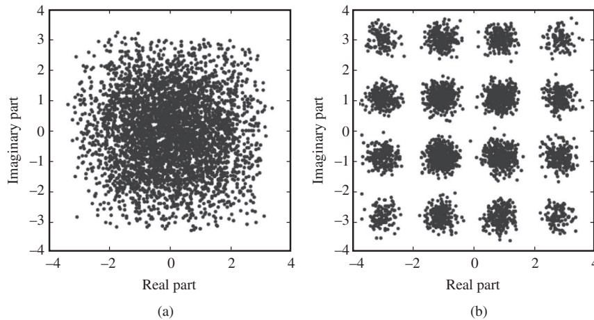
Figure 11.22 Scatter plots of signal samples before (a) and after (b) linear equalization at E_b/\mathcal{N} = 26 dB demonstrate effective ISI mitigation by the linear equalizer.
