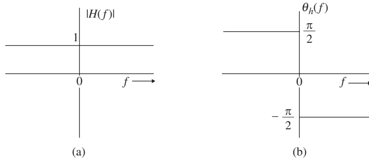
Figure 4.13 Transfer function of an ideal \pi/2 phase shifter (Hilbert transformer).
