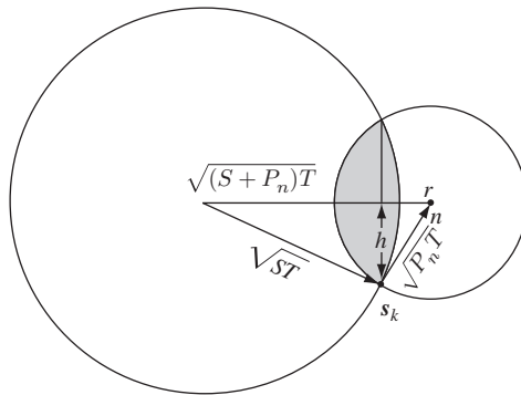
Figure 12.8 Derivation of channel capacity.
