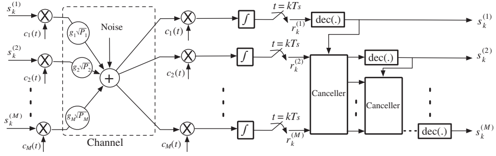
Figure 10.16 Decision feed- back MUD receiver based on successive interference cancellation (assuming that all M users are ranked in the order of descending gains).
