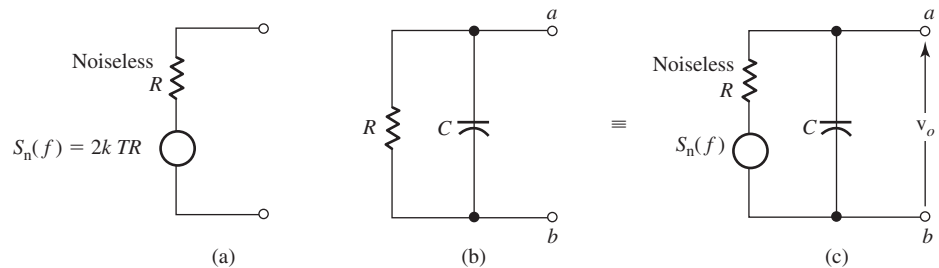
Figure 8.13 Representation of thermal noise in a resistor.
