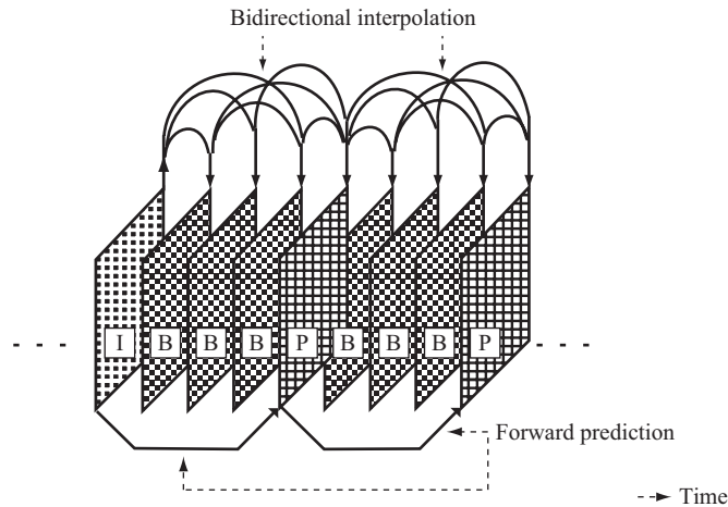
Figure 5.40 MPEG temporal frame structure.
