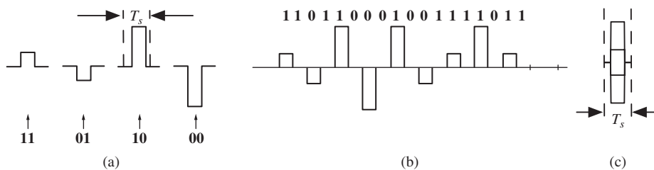
Figure 6.28 4-Ary PAM signaling: (a) four RZ symbols; (b) baseband transmission; (c) the 4-ary RZ eye diagram.
