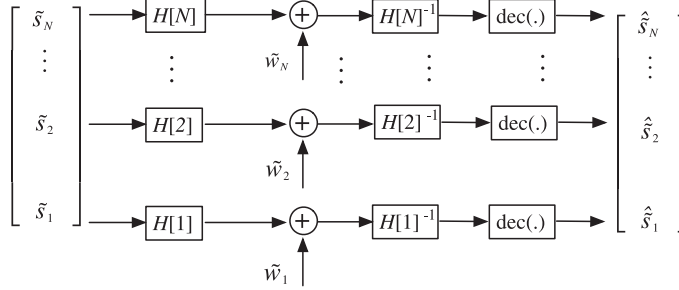
Figure 11.12 Using a bank of receiver gain adjusters for N independent AWGN channels in OFDM to achieve gain equalization.
