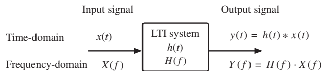
Figure 3.24 Signal transmission through a linear time-invariant system.
