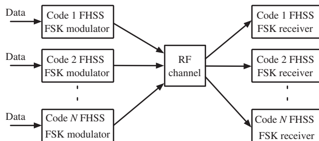
Figure 10.4 CDMA in FHSS in which each of the M users is assigned a unique PN code.
