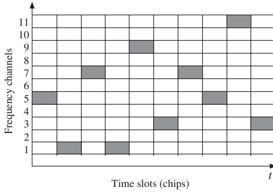
Figure 10.2 Typical Bluetooth frequency hopping pattern.
