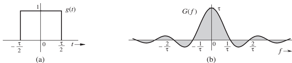
Figure 3.8 (a) Rectangular pulse and (b) its Fourier spectrum.
