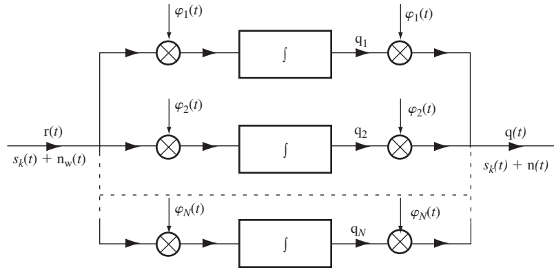
Figure 9.16 Eliminating the noise orthogonal to signal space.
