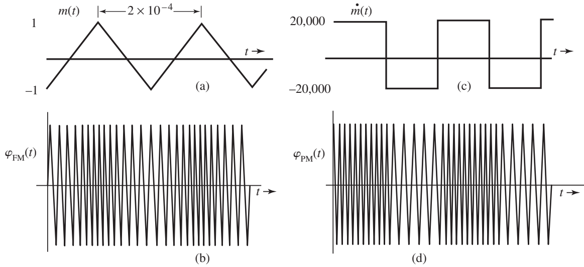
Figure 4.25 FM and PM waveforms.
