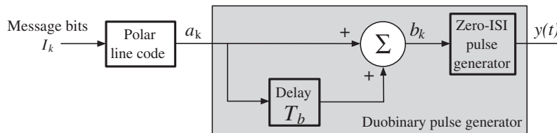
Figure 6.17 Equivalent duobinary signaling.
