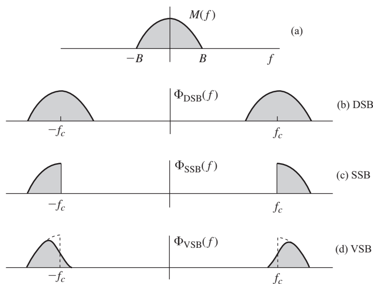
Figure 4.18 Spectra of the modulating signal and corresponding DSB, SSB, and VSB signals.
