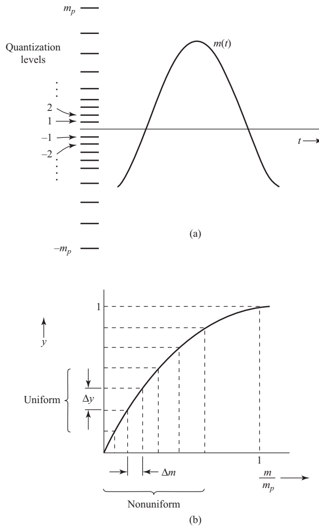
Figure 5.16 Nonuniform quantization.
