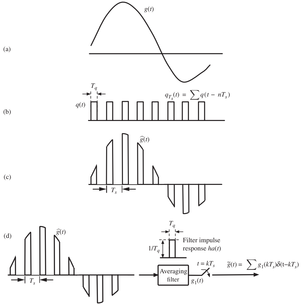
Figure 5.11 Illustration of practical sampling.
