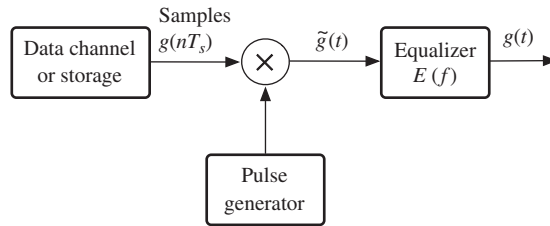
Figure 5.5 Diagram for practical signal reconstruction.
