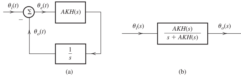
Figure 4.37 Equivalent circuits of a linearized PLL.
