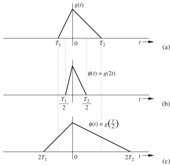
Figure 2.7 Time scaling a signal.
