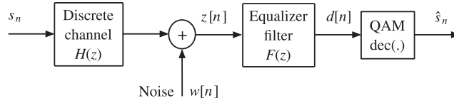
Figure 11.5 A SISO discrete linear channel model for TSE.
