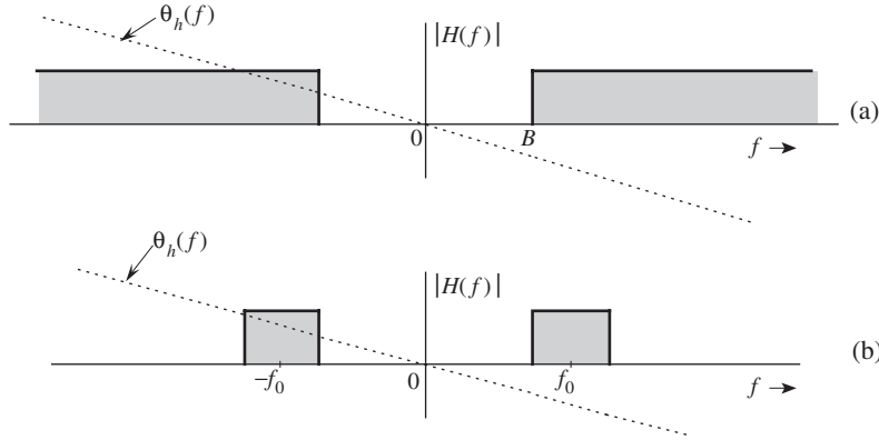
Figure 3.28 Frequency responses of (a) ideal highpass filter and (b) ideal bandpass filter.
