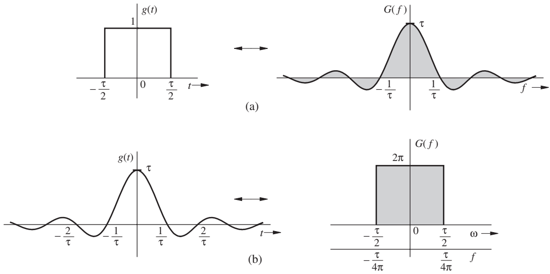
Figure 3.14 Duality property of the Fourier transform.
