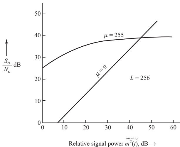
Figure 5.19 Ratio of signal to quantization noise in PCM with and without compression.
