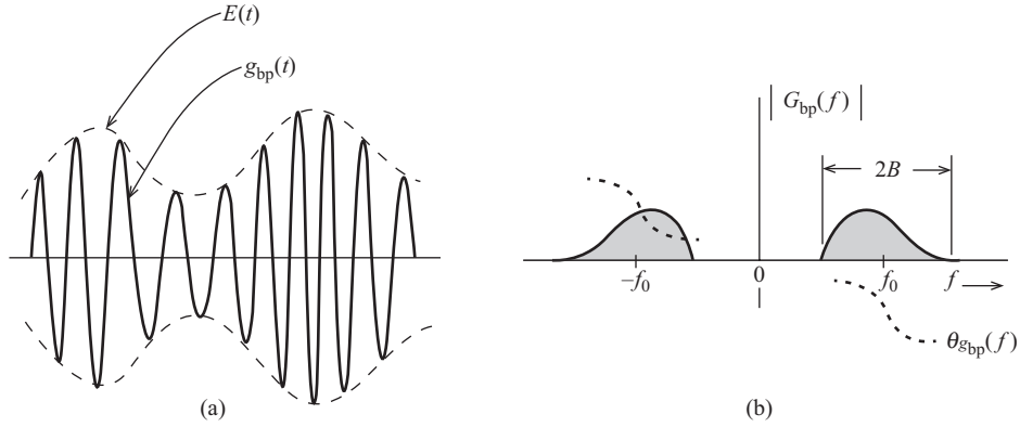
Figure 3.21 (a) Bandpass signal and (b) its spectrum.
