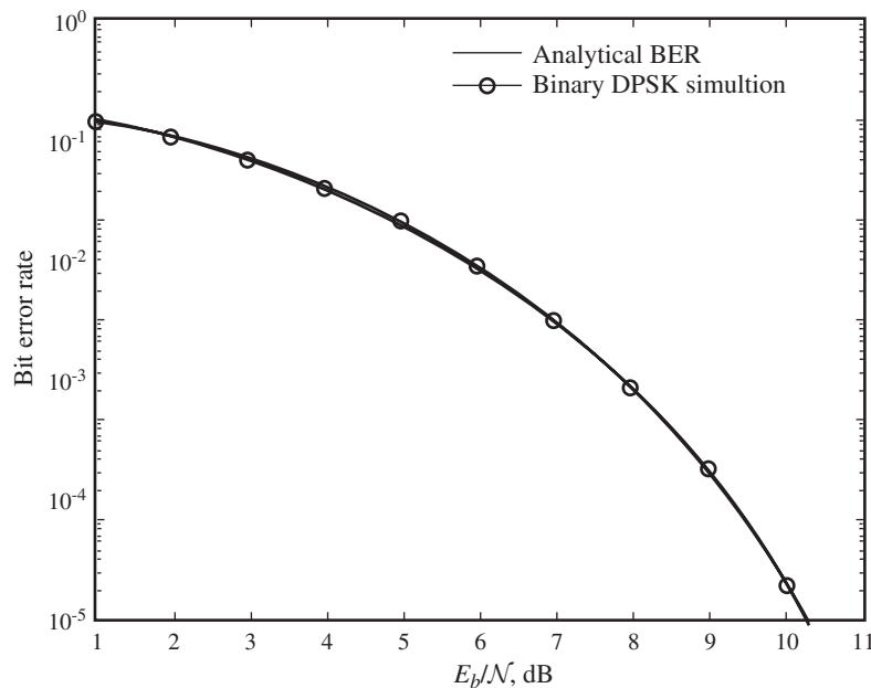
Figure 9.51 Analytical BER results from noncoherent detection of binary DPSK simulation (round points).
