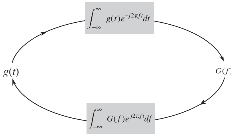
Figure 3.13 Near symmetry between direct and inverse Fourier transforms.
