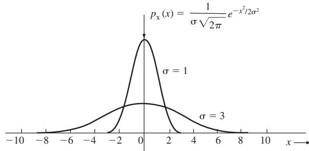
Figure 7.17 Gaussian PDF with standard deviations \sigma = 1 and \sigma = 3 .
