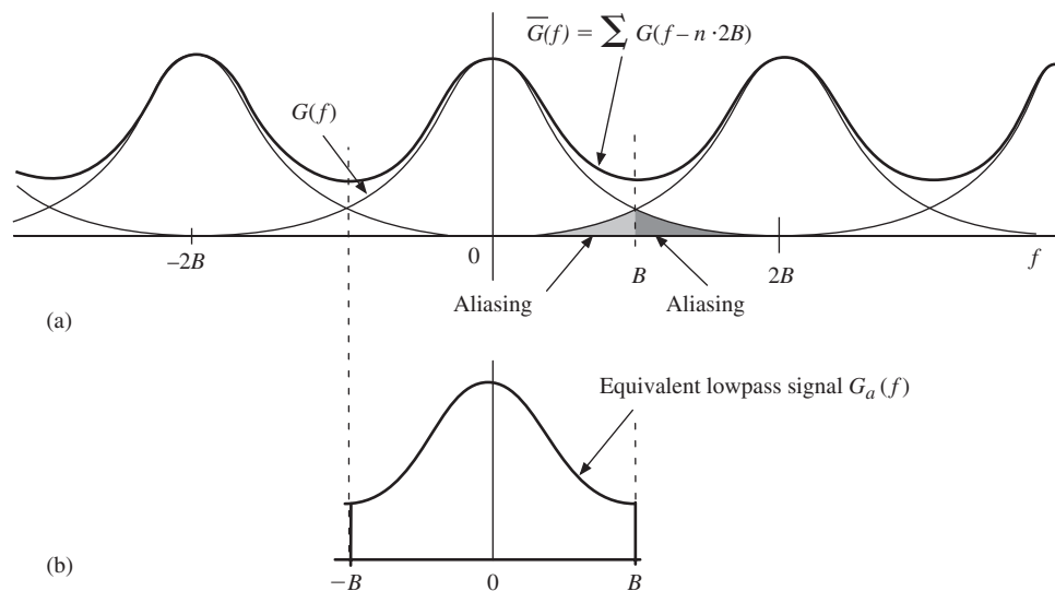
Figure 5.10 (a) Non-bandlimited signal spectrum and its sampled spectrum \bar{G}(f) . (b) Equivalent lowpass signal spectrum G_a(f) constructed from uniform samples of g(t) at sampling rate 2B .
