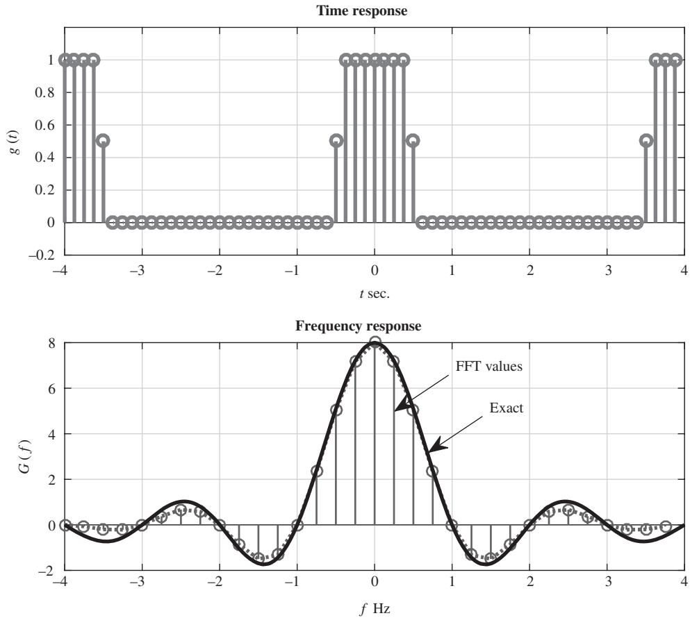
Figure 3.46 Discrete Fourier transform of a rectangular pulse.
