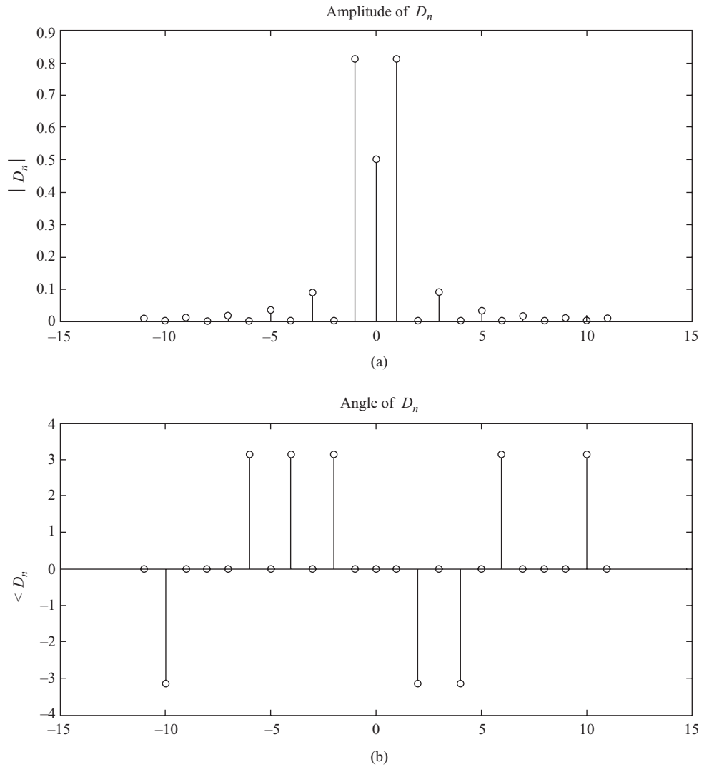
Figure 2.31 Exponential Fourier series coefficients of a repeated \Delta(t/2) with period T = 4 showing (a) amplitude and (b) angle of D_n .
