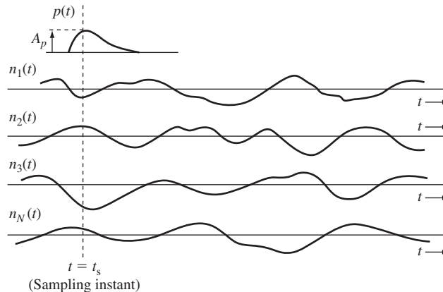
Figure 8.3 Random process for representing a channel noise.
