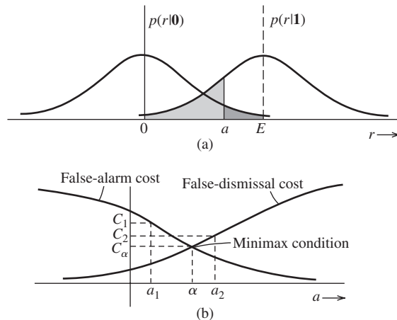
Figure 9.34 Explanation of minimax concept.
