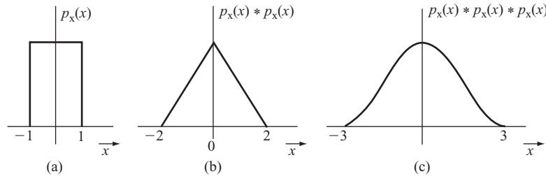
Figure 7.20 Demonstration of the central limit theorem.
