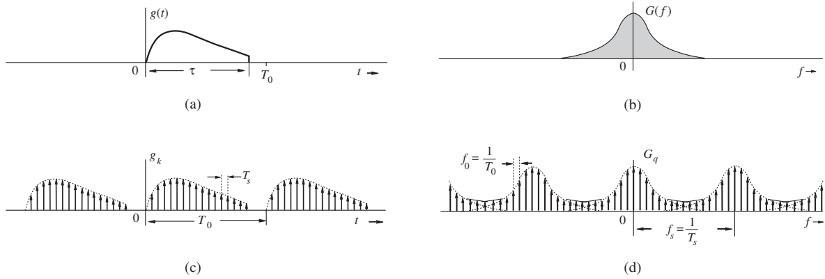
Figure 3.44 Relation between the samples of g(t) and of G(f) .
