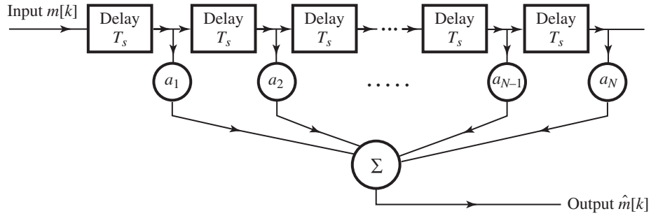
Figure 5.28 Transversal filter (tapped delay line) used as a linear predictor.
