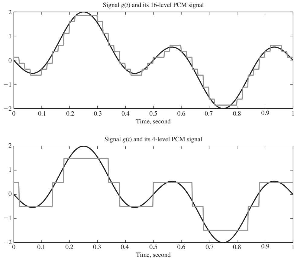
Figure 5.44 Original signal and the PCM signals with different numbers of quantization levels.
