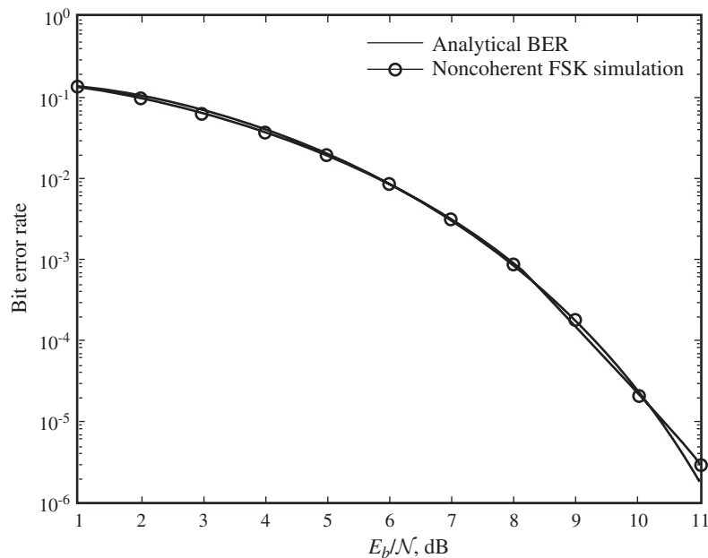
Figure 9.50 BER from noncoherent detection of binary FSK.
