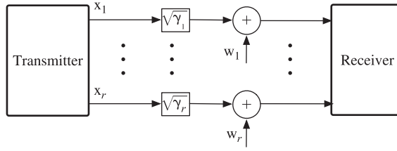
Figure 12.11 r -Channel communication system equivalent to a MIMO system without channel knowledge at the transmitter.
